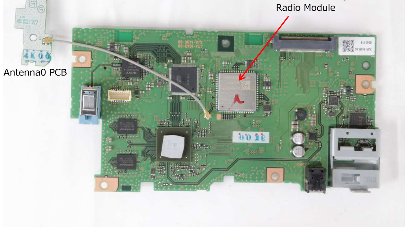
PCB(A-side) with Radio module
