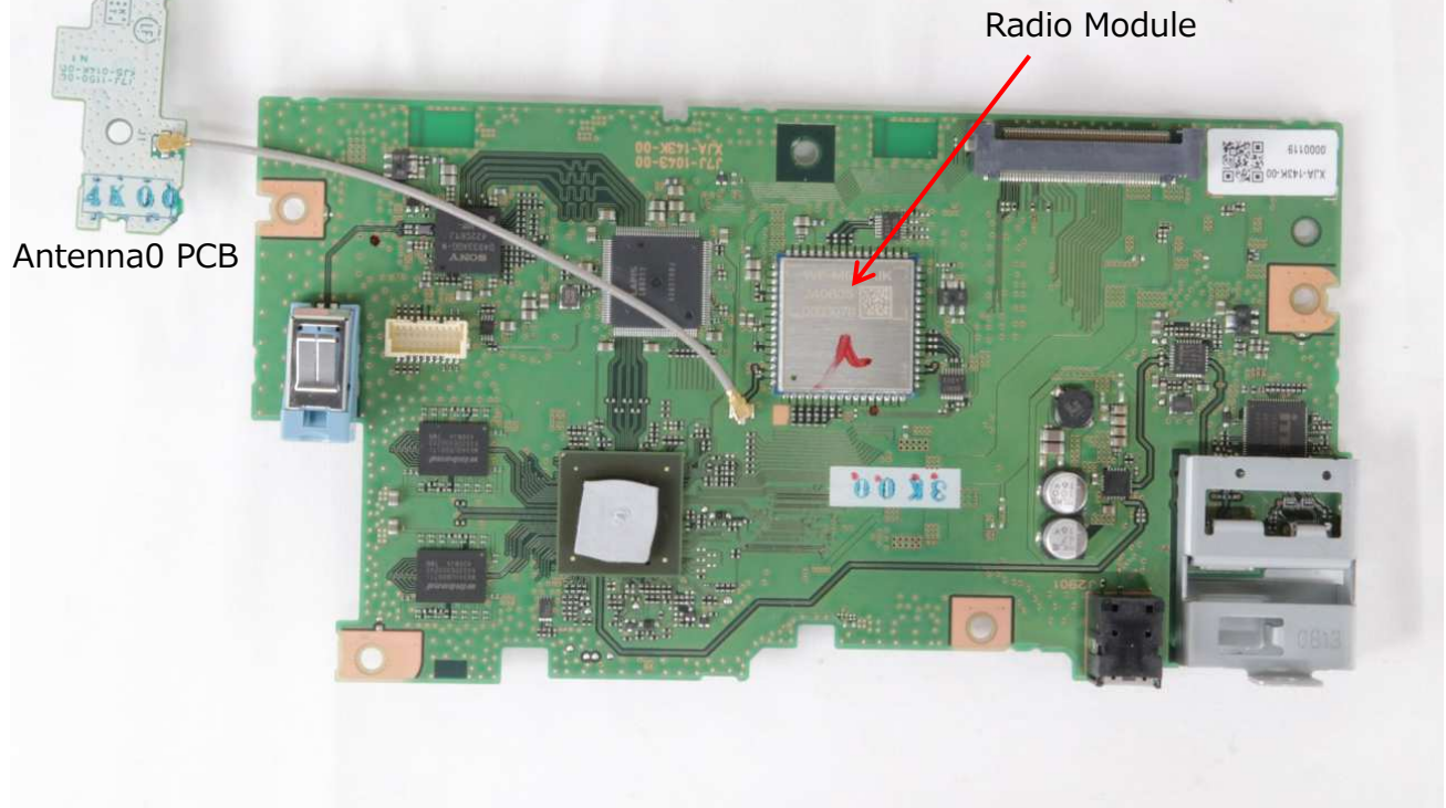
PCB(A-side) with Radio module
