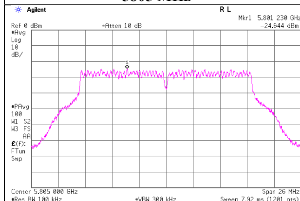
5805 MHz
