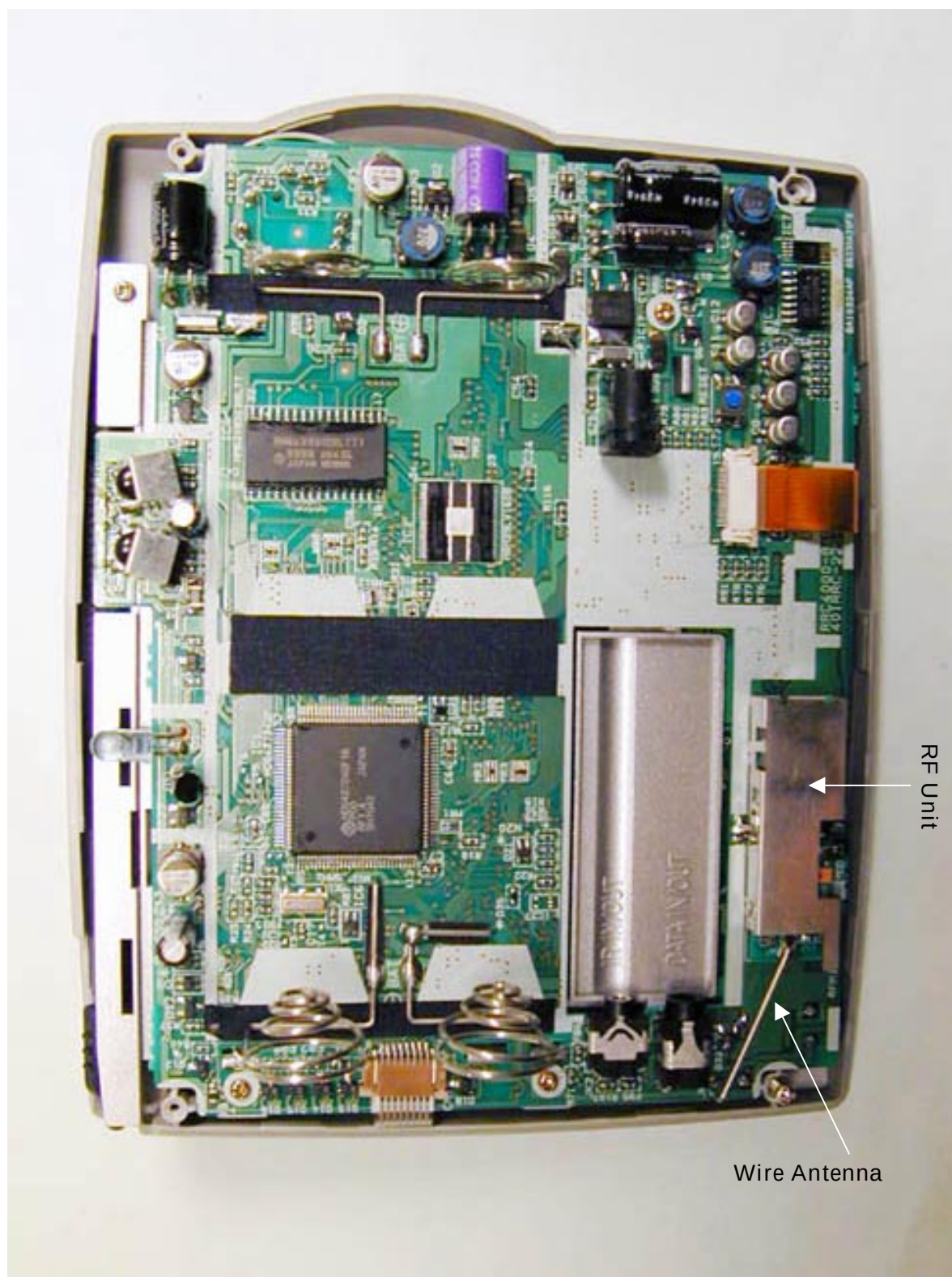
Fig.E-3 Internal View of RC-R1110
