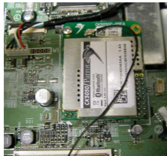
Bluetooth ANTENNA-1
