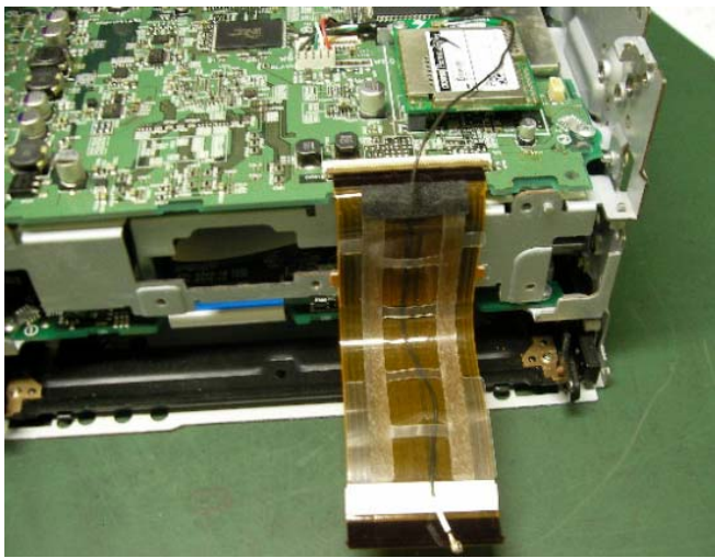
Bluetooth ANTENNA-2
