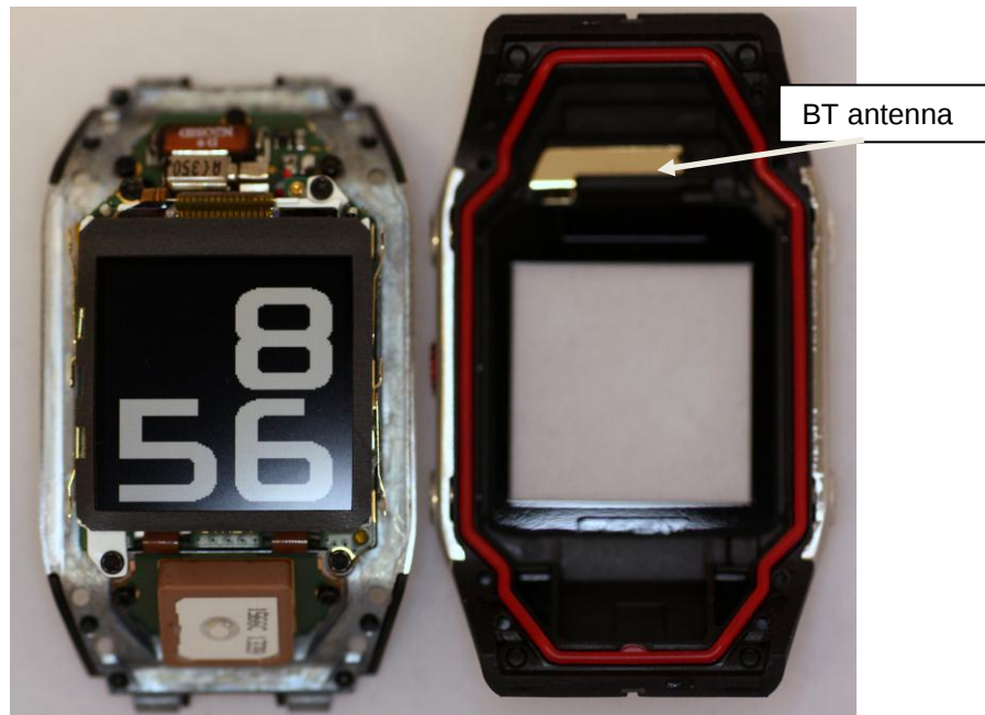
Figure 1. Front cover opened
