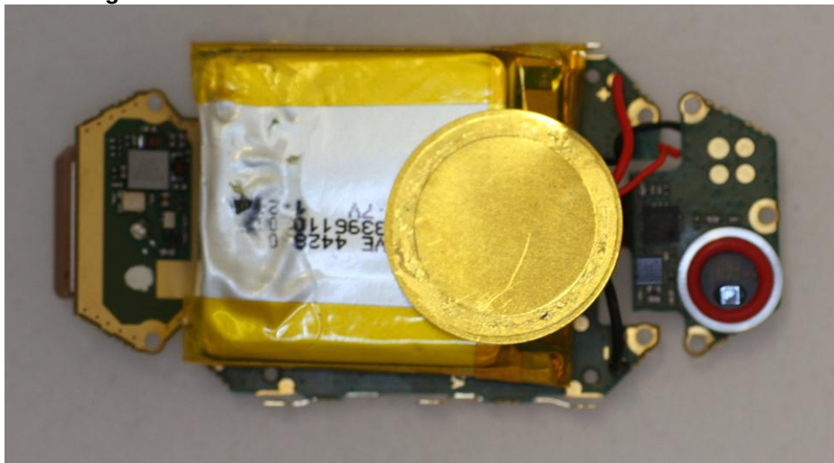
Figure 4. Electronics module from the back side. Battery and piezo element of top of PWB.
