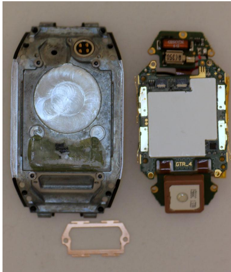
Figure 3. Electronics module detached from the back cover.
