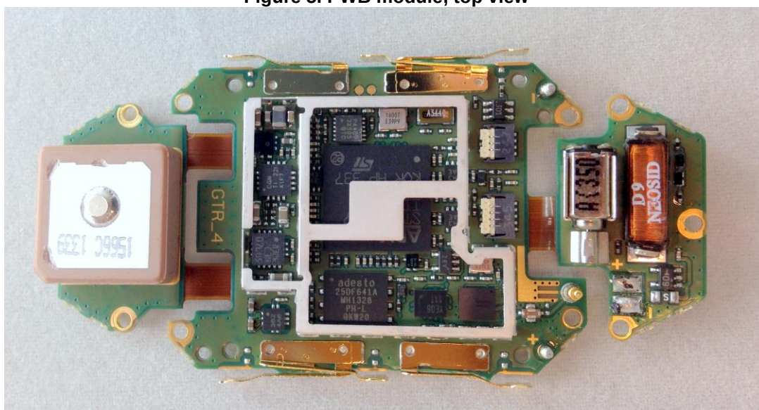
Figure 6. PWB module shield opened, top view.
