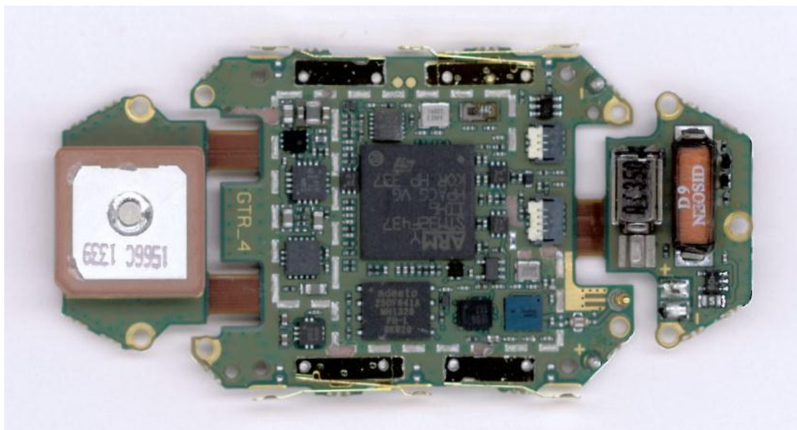
Figure 7. PWB module shield removed, top view.
