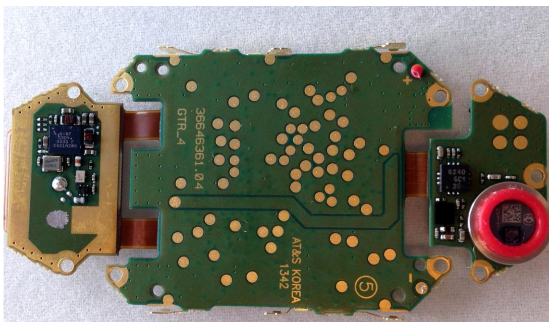
Figure 8. PWB module from the backside.
