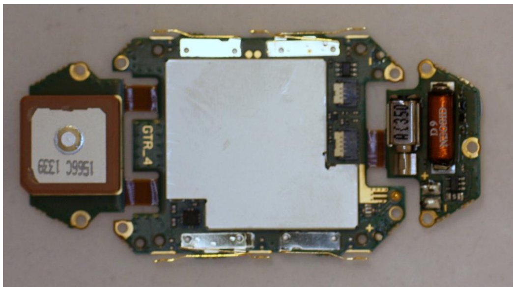
Figure 5. PWB module, top view
