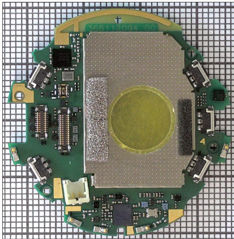
Figure 7. The main PWB from component side with RF shield on.
