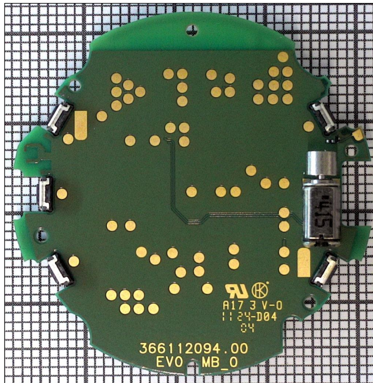
Figure 9. The main PWB from bottom side.
