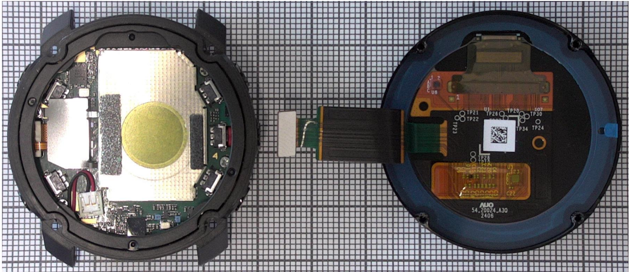
Figure 3. Display module separated.
