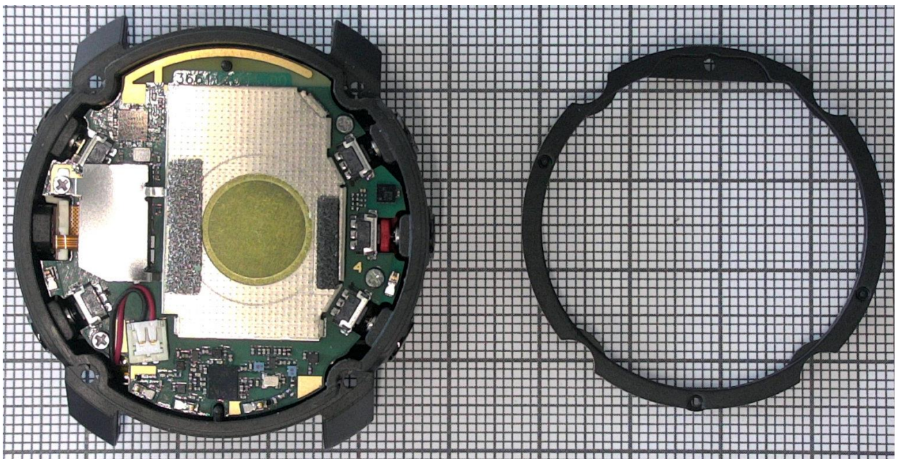
Figure 4. Antenna frame separated.
