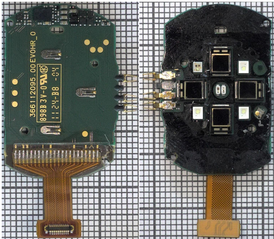
Figure 14. OHR PWB from component side and LED side.
