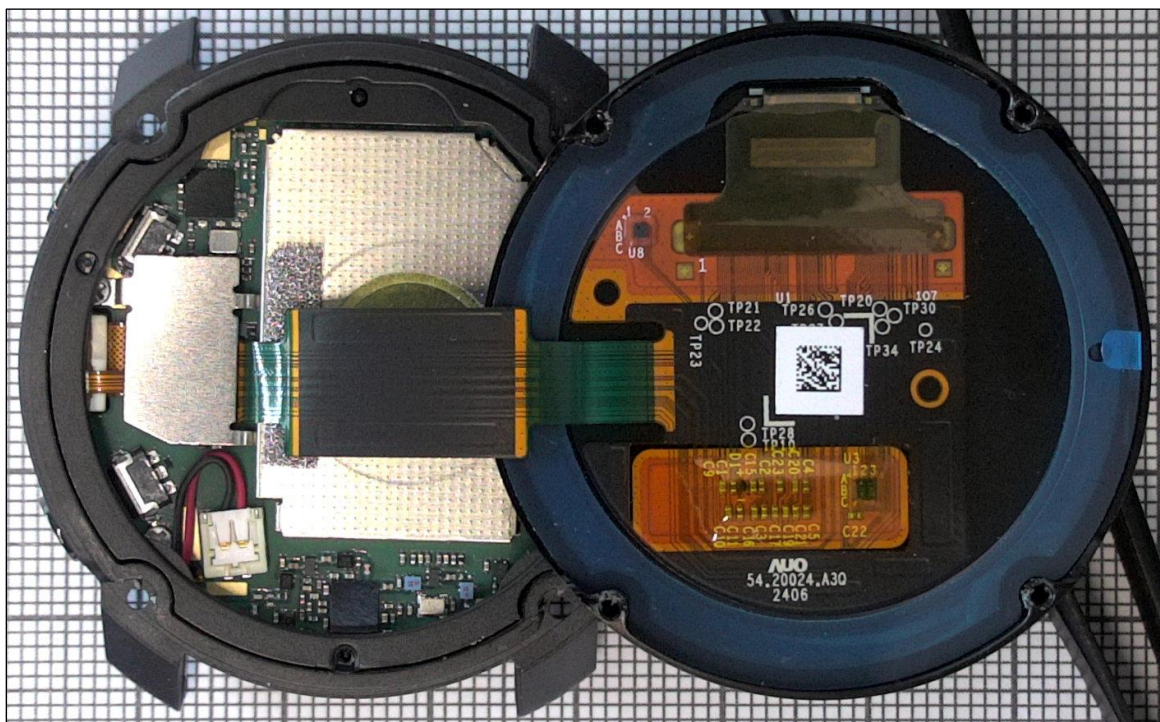
Figure 2. Device opened, display cable attached.
