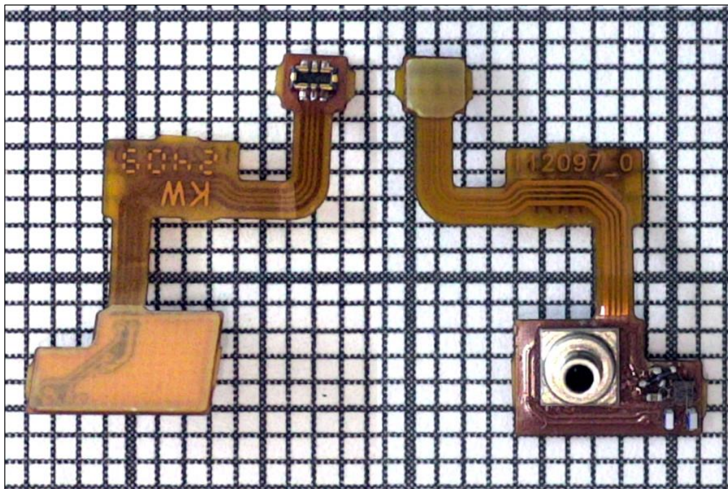
Figure 16. Barometer PWB from both sides.
