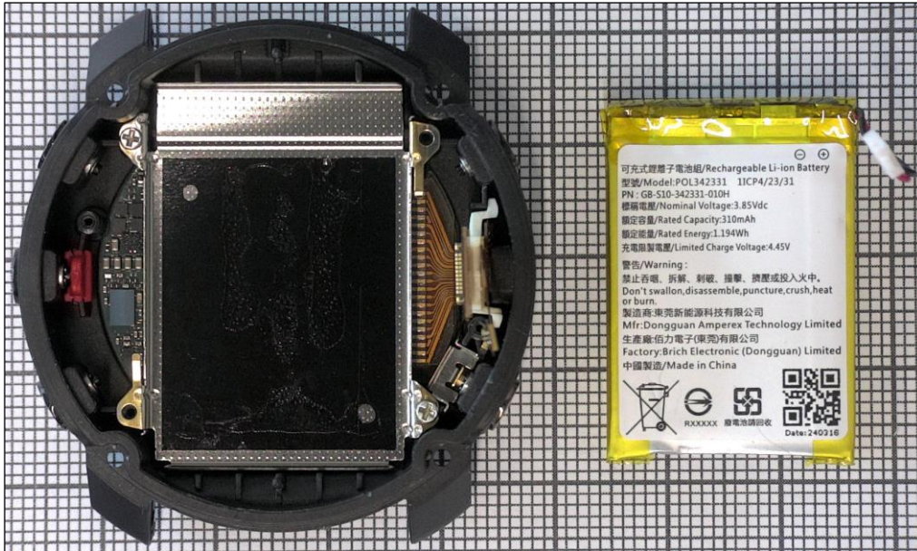
Figure 11. Battery removed, battery shield visible.
