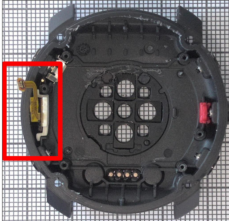
Figure 15. Barometer PWB location.
