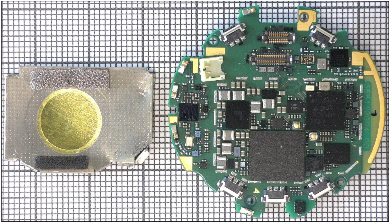
Figure 8. The main PWB from component side with RF shield removed.
