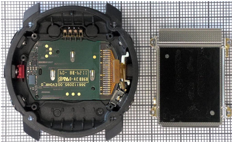
Figure 12. Battery shield removed, OHR PWB visible.
