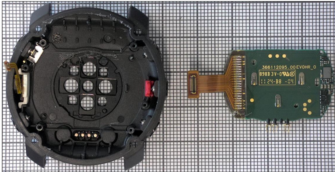
Figure 13. OHR PWB removed from the case.
