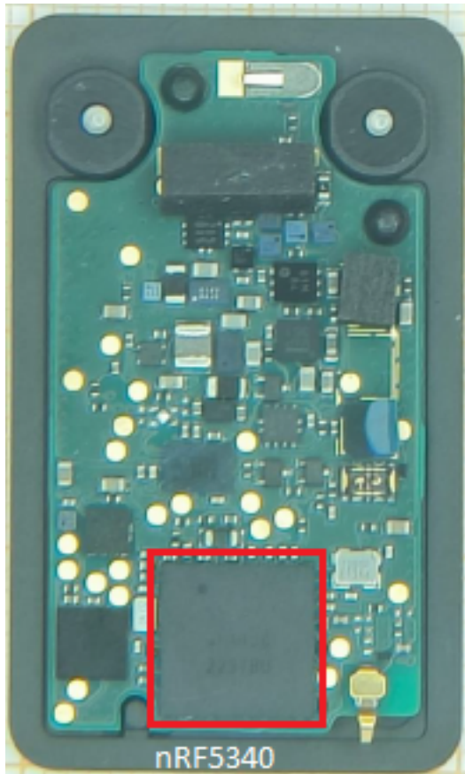
Figure 4. PWB from component side.
