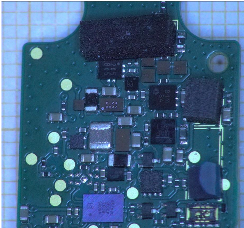
Figure 6. PWB enlarged from component. Picture from the USB-contacts end.
