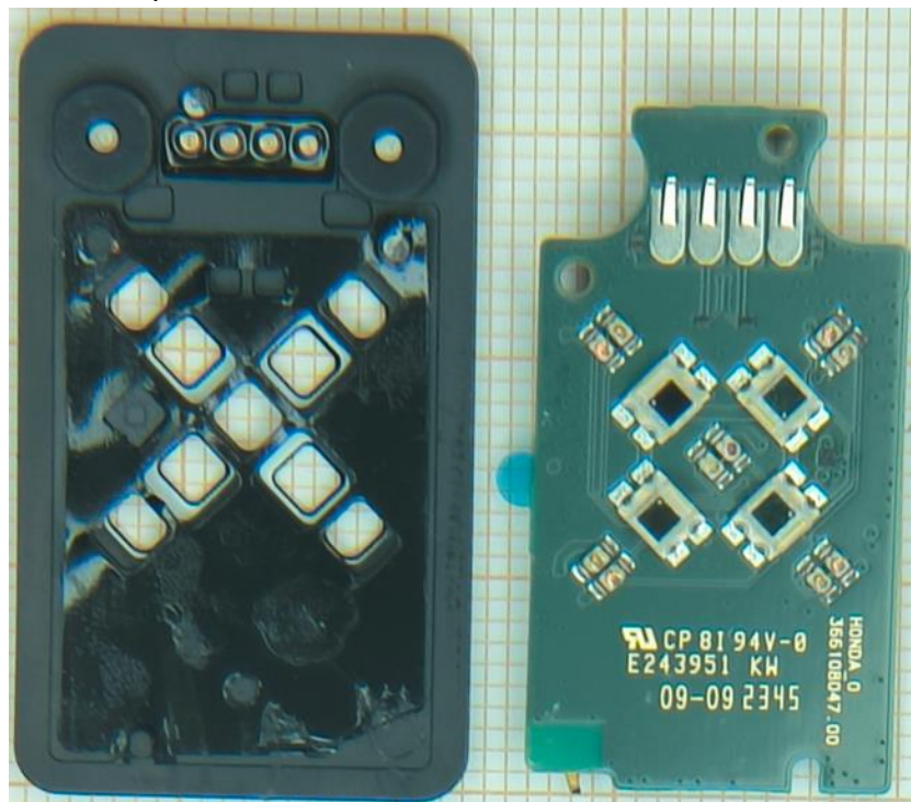
Figure 3. Battery removed
