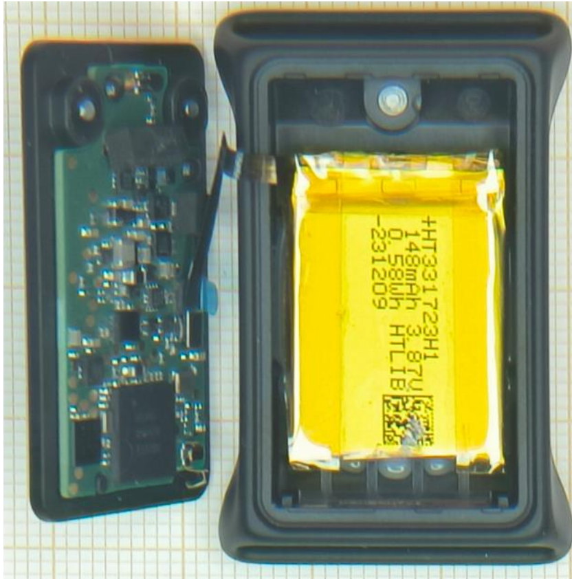
Figure 1. Device opened, F.case and B.case separated.
