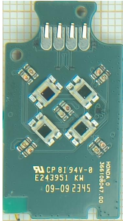
Figure 5. PWB from OHR LED side
