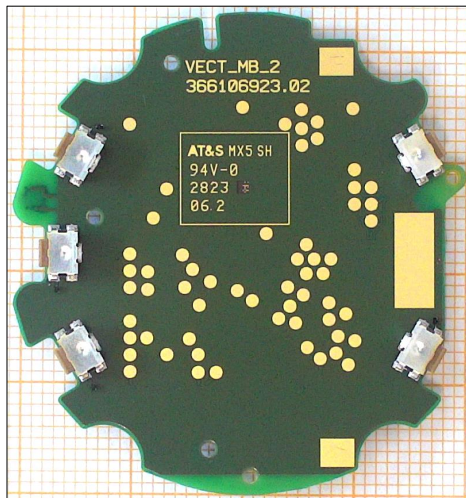
Figure 7. The main PWB from bottom side.
