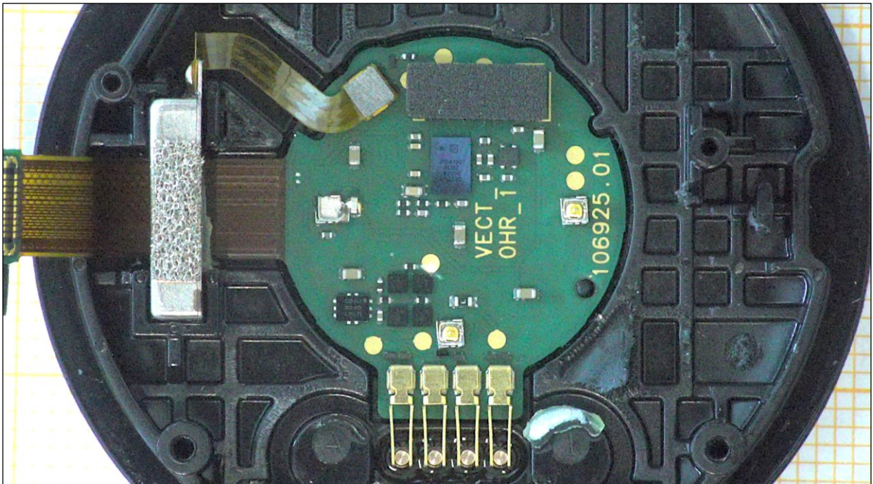
Figure 10. OHR assembly details.
