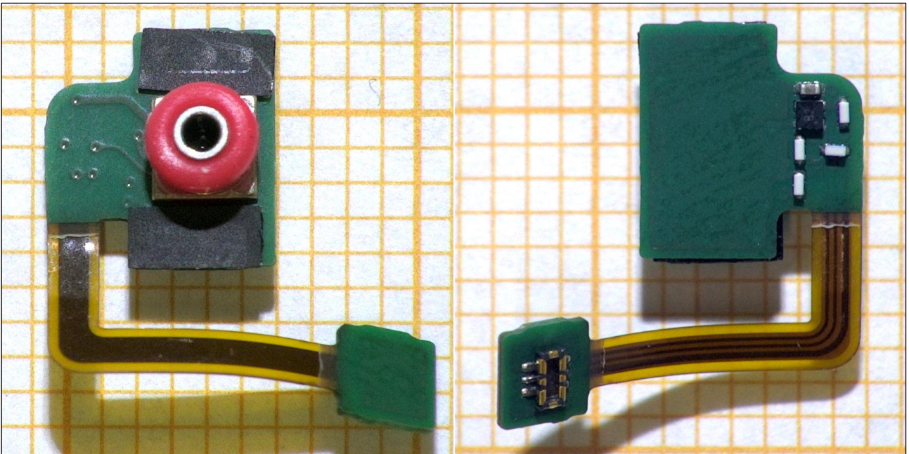
Figure 16. Barometer PWB on both sides.
