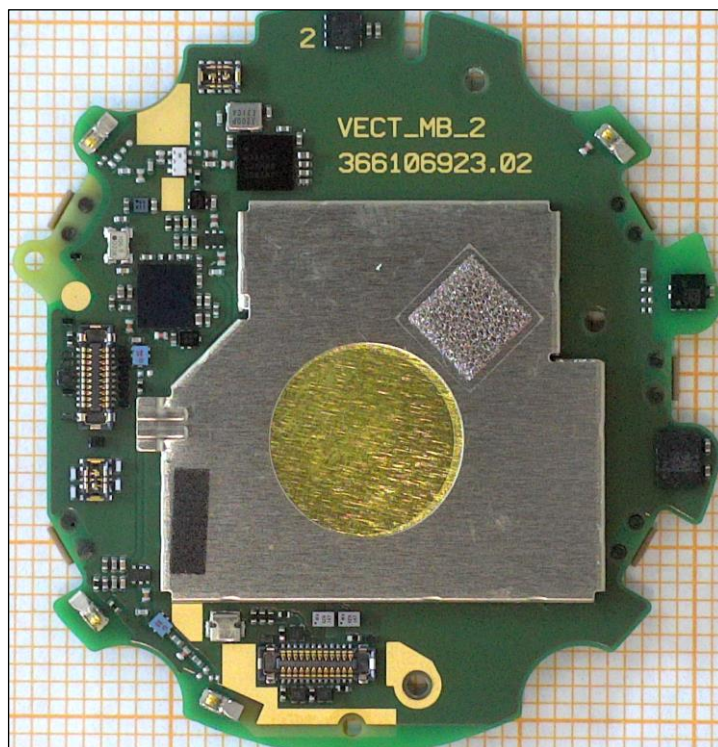
Figure 5. The main PWB from component side with RF shield on.
