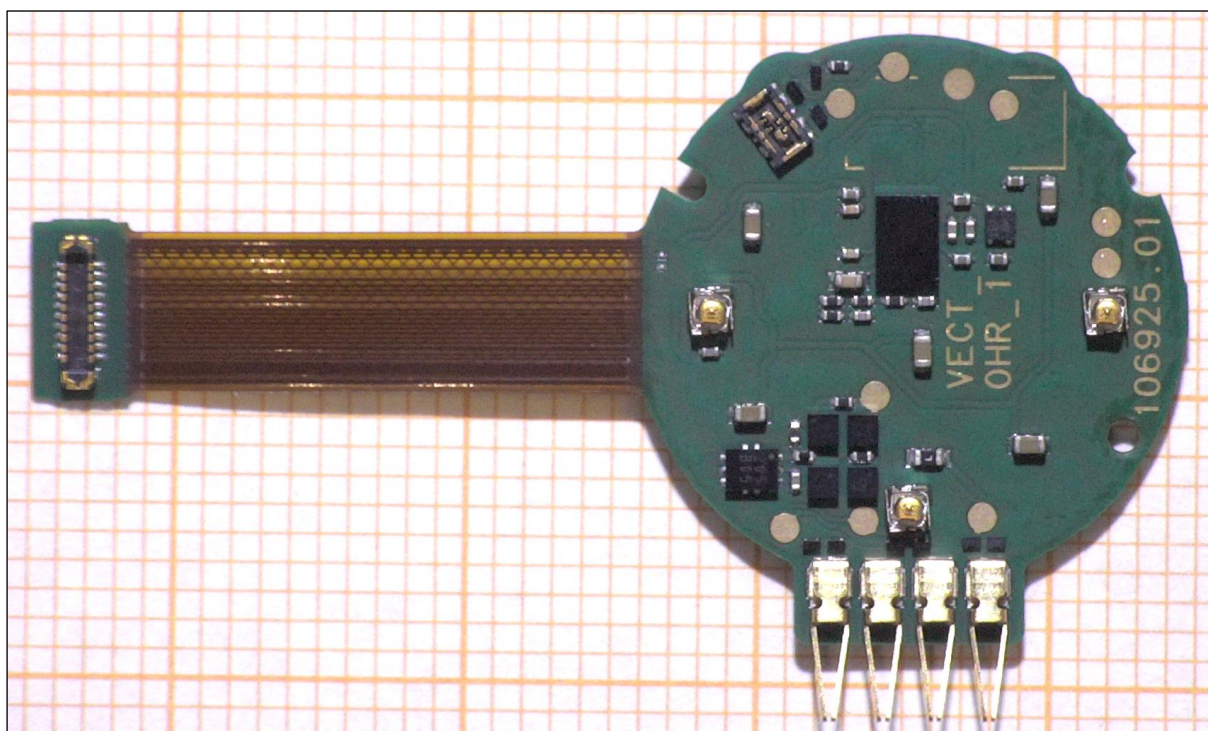
Figure 12. OHR PWB from component side.
