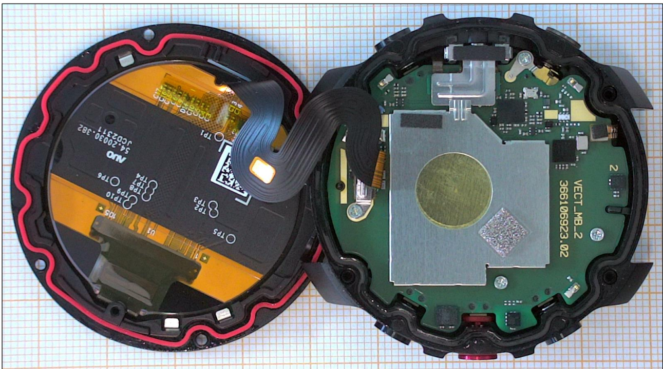
Figure 2. Device opened, display cable attached.
