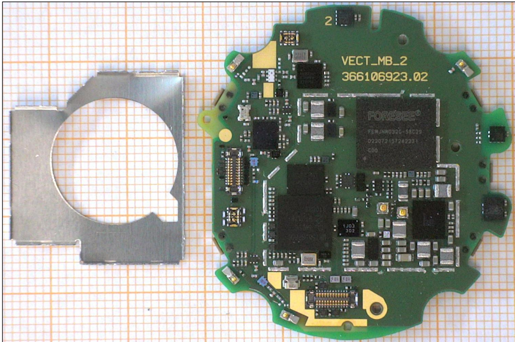
Figure 6. The main PWB from component side with RF shield removed.
