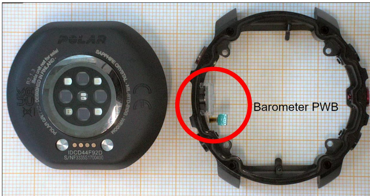
Figure 14. Device case and bottom case separated. Barometer PWB visible.
