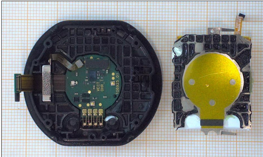
Figure 9. Battery removed, OHR PWB visible.
