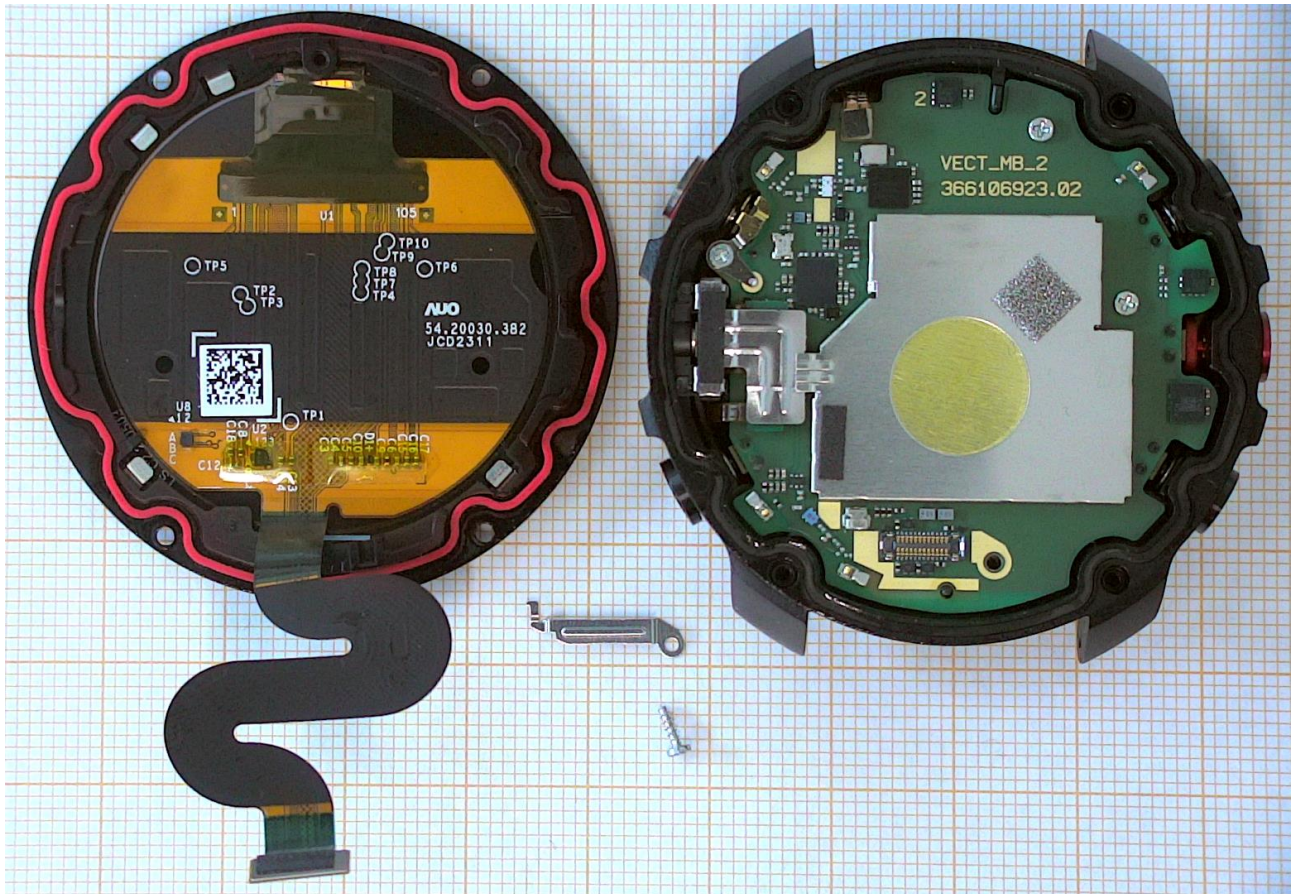
Figure 3. Display module separated.
