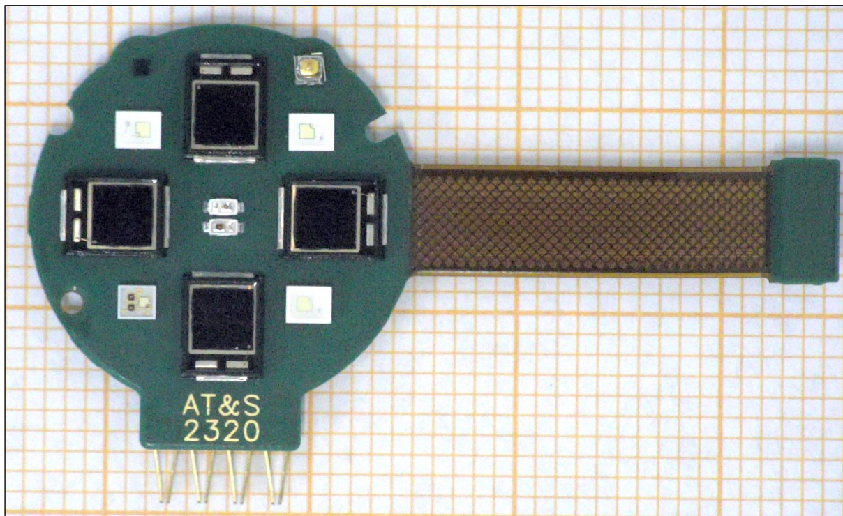
Figure 11. OHR PWB from LED side.
