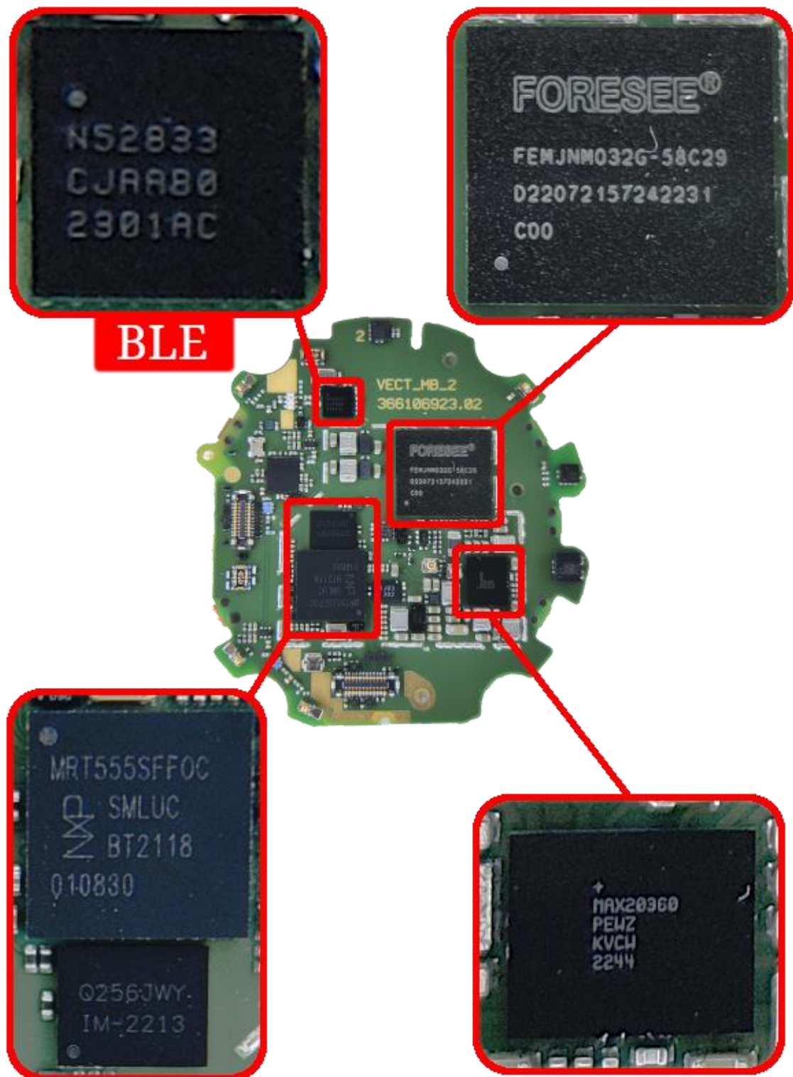
Figure 8. Main PWB component details.
