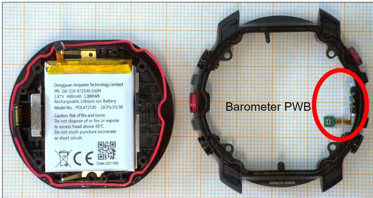
Figure 13. Device case and bottom case separated. Barometer PWB visible.
