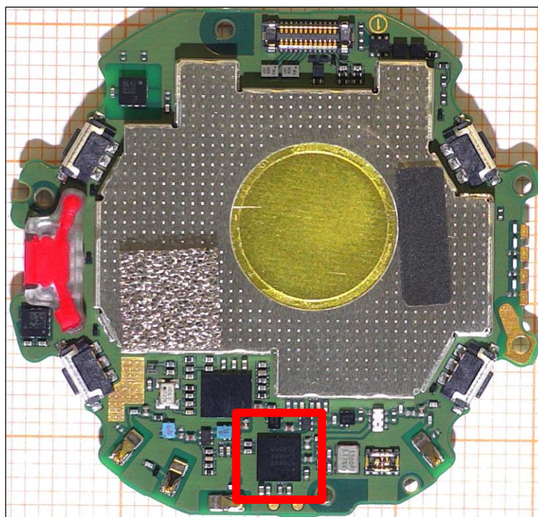
Figure 4. The main PWB from component side with RF shield on. BLE chipset in red frame.
