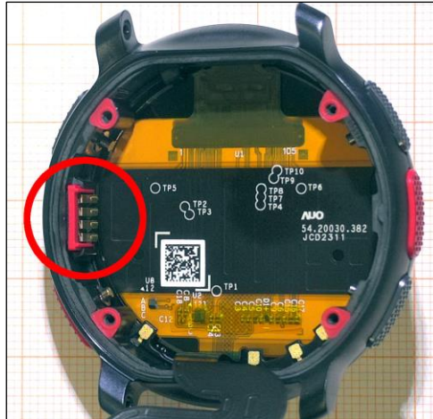
Figure 13. Barometer PWB location.
