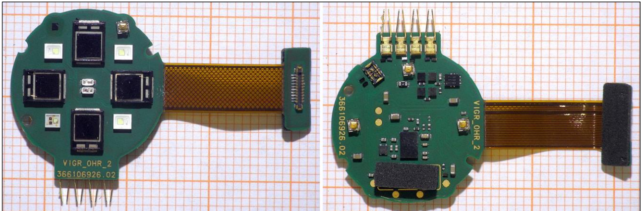
Figure 11. Left: OHR PWB from LED side. Right: OHR PWB from component side.
