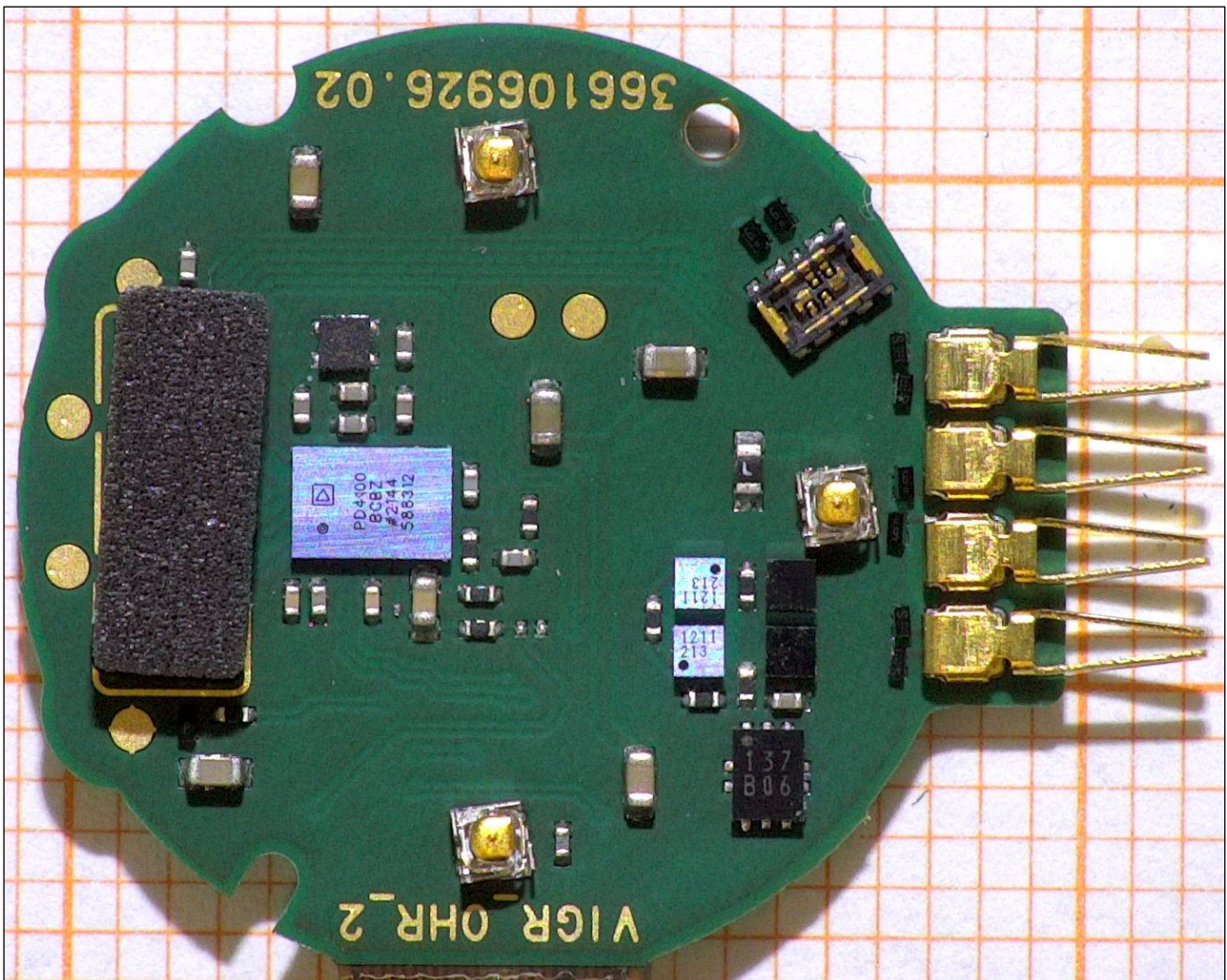
Figure 12. OHR PWB component details.
