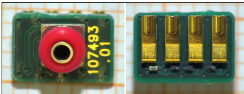
Figure 15. Barometer PWB on both sides.
