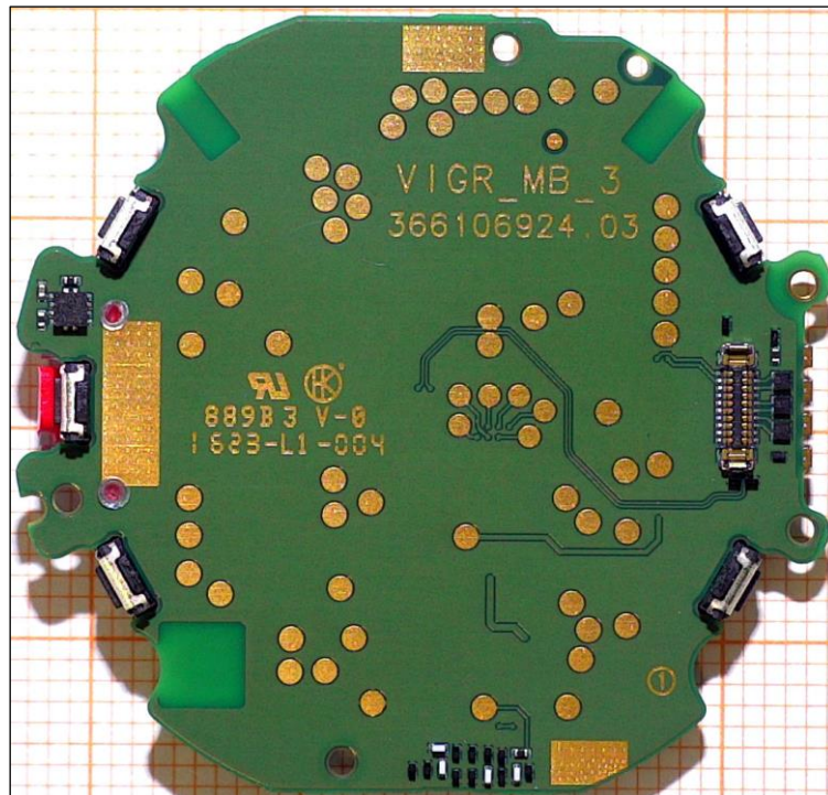
Figure 6. The main PWB from bottom side.
