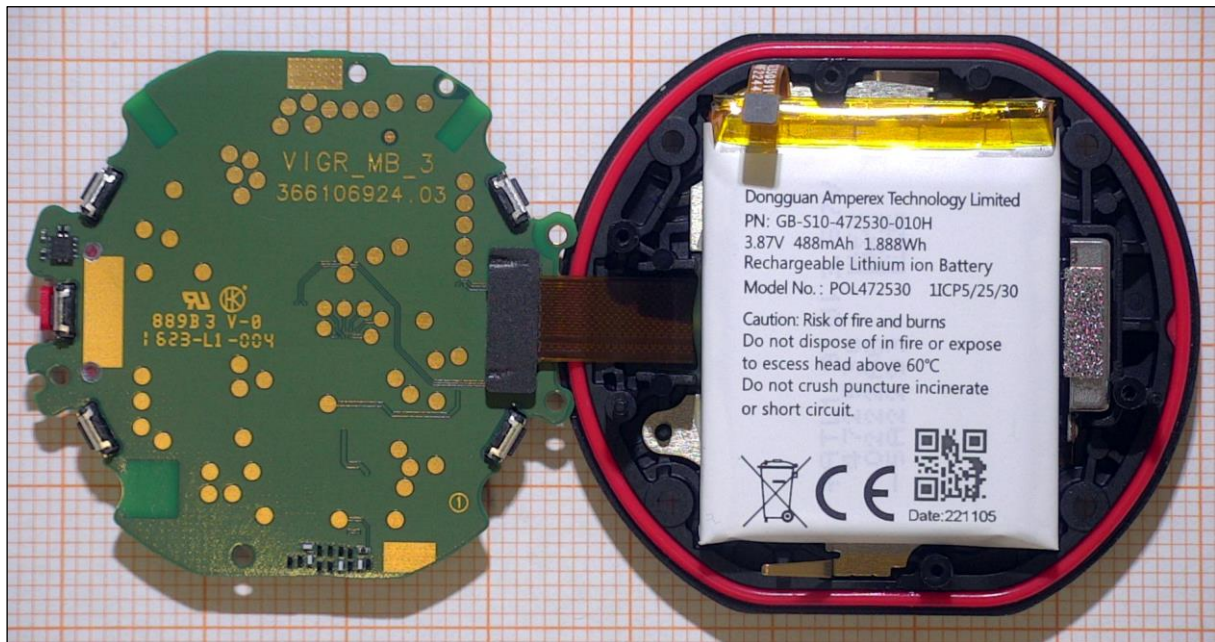
Figure 3. The main PWB removed.
