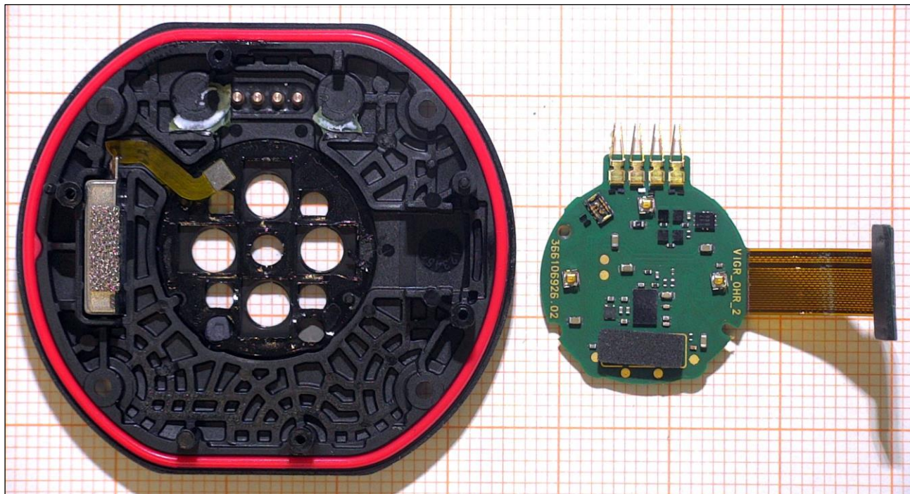
Figure 10. OHR PWB removed.
