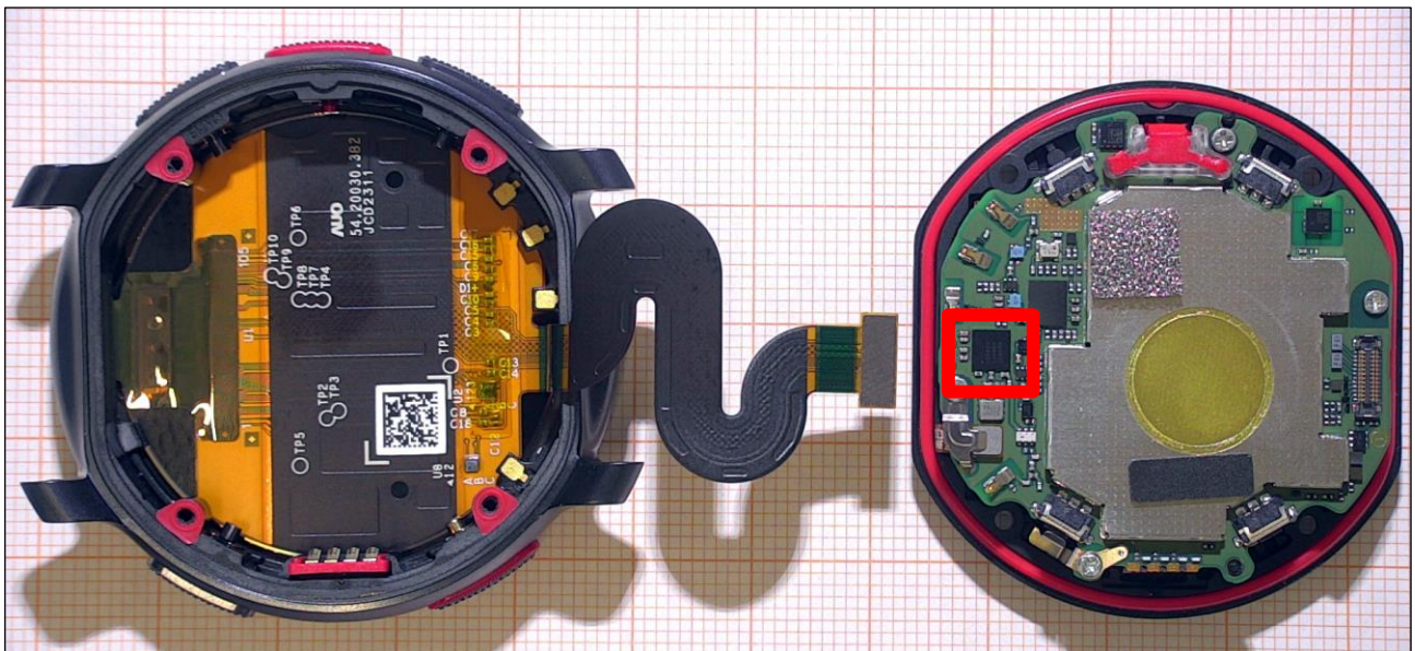
Figure 2. The display module separated. BLE chipset in red frame.
