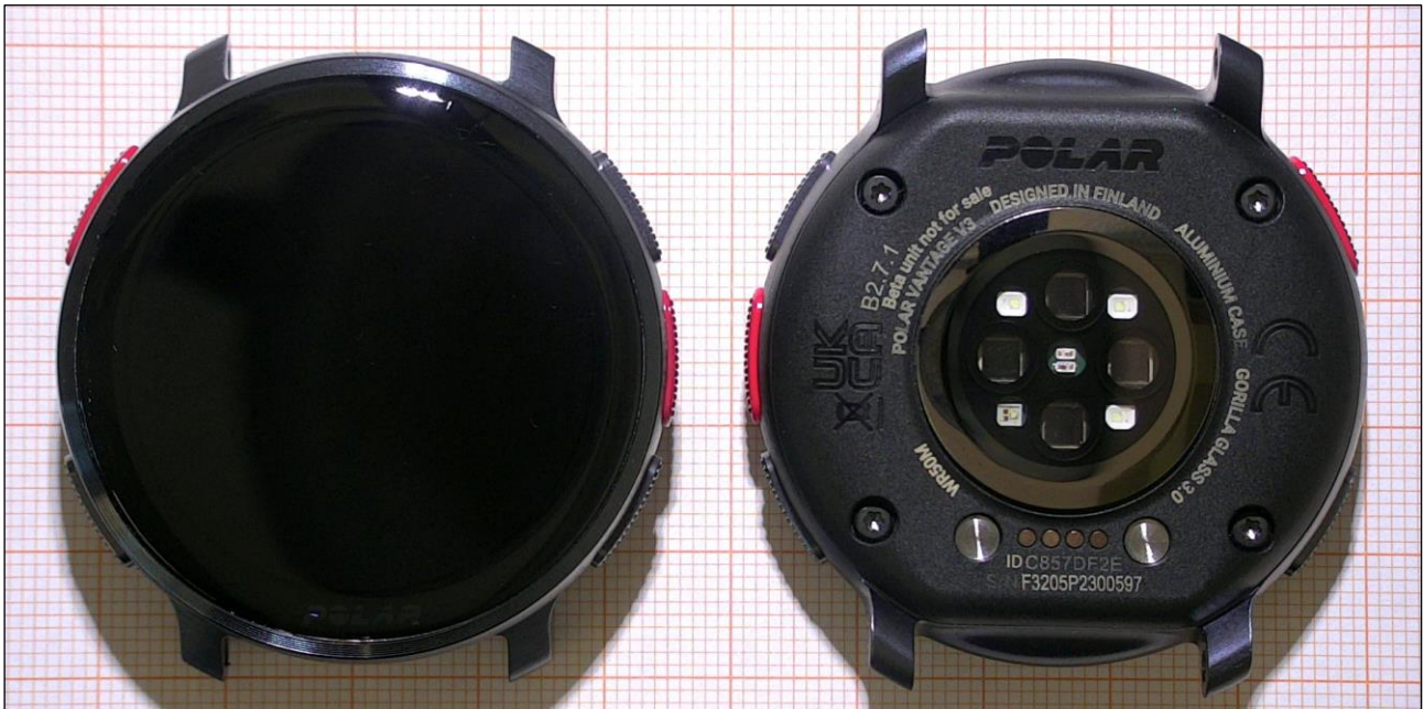
Figure 1. Whole device from both sides.
