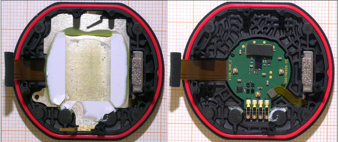
Figure 9. Left: Battery removed, shield visible. Right: Shield removed, OHR PWB visible.
