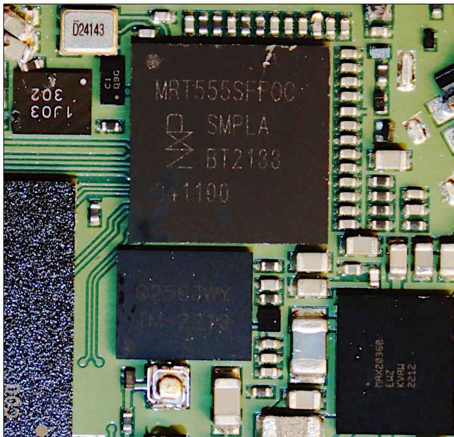
Figure 8. Main PWB component details 2.
