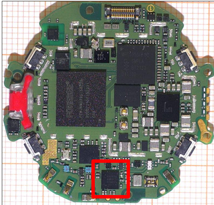
Figure 5. The main PWB from component side with RF shield removed. BLE chipset in red frame.
