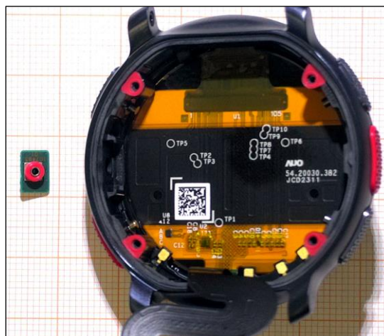
Figure 14. Barometer PWB removed.
