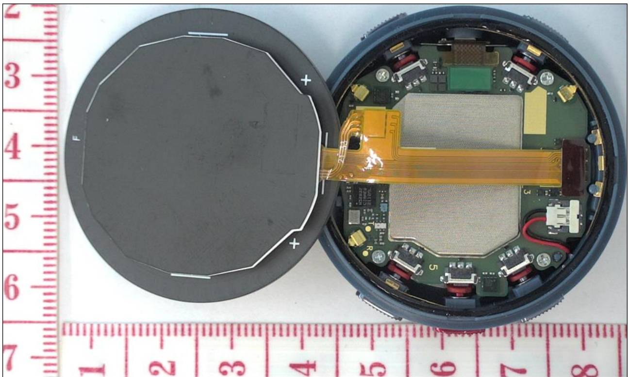
Figure 2. The display module separated.
