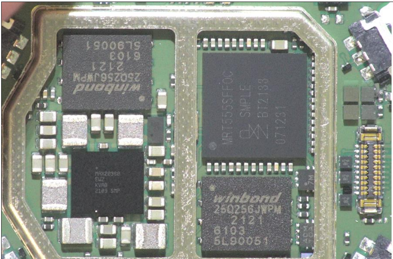
Figure 7. Component details 1.
