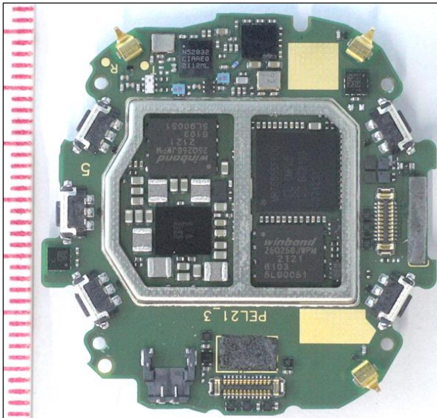
Figure 5. The main PWB from component side.
