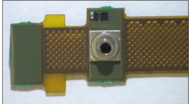
Figure 10. OHR PWB component details 2.
