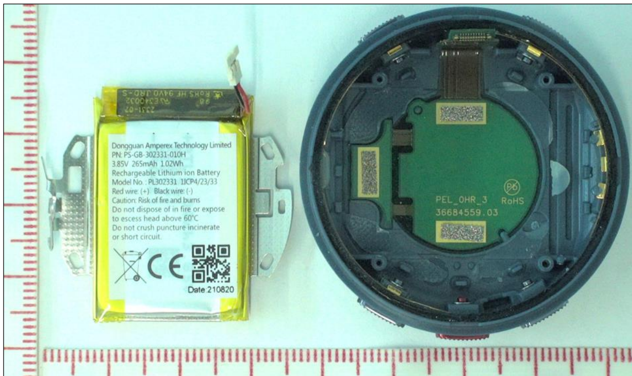
Figure 9. Battery removed and OHR PWB visible.
