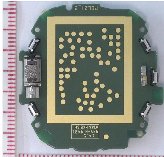
Figure 6. The main PWB from vibra motor side.
