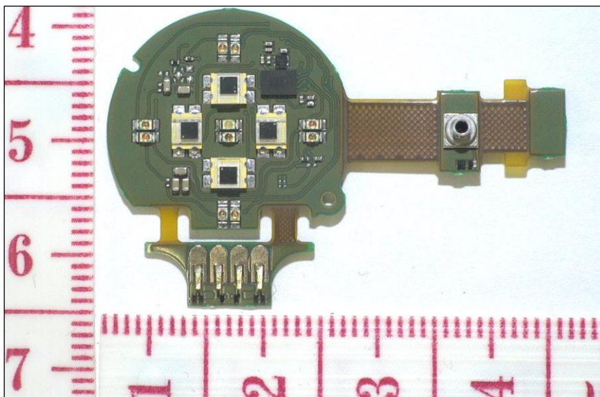
Figure 11. OHR PWB from component side.
