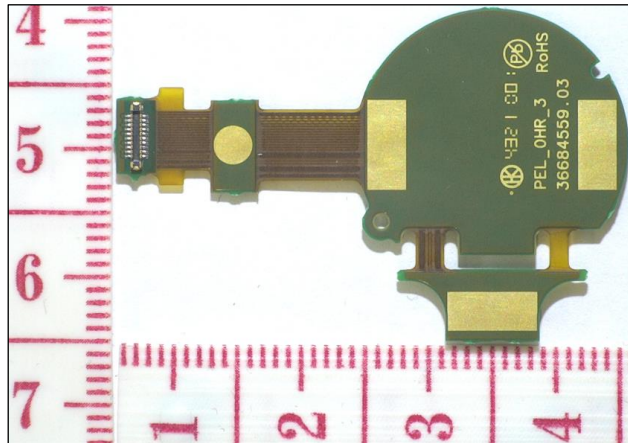
Figure 114. OHR PWB from other side.
