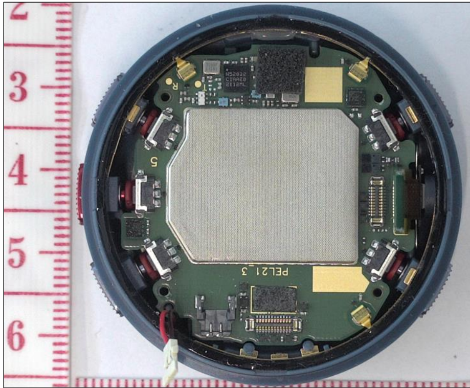
Figure 3. The connectors screws have been removed.
