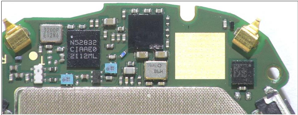
Figure 8. Component details 2.
