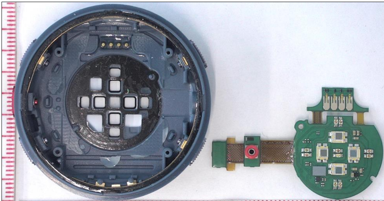
Figure 10. OHR PWB removed.
