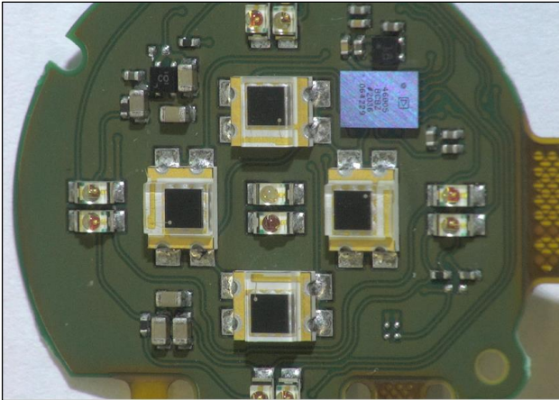
Figure 12. OHR PWB component details 1.
