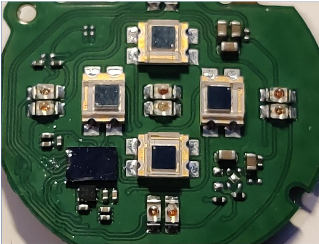
Figure 13. OHR PWB component details.
