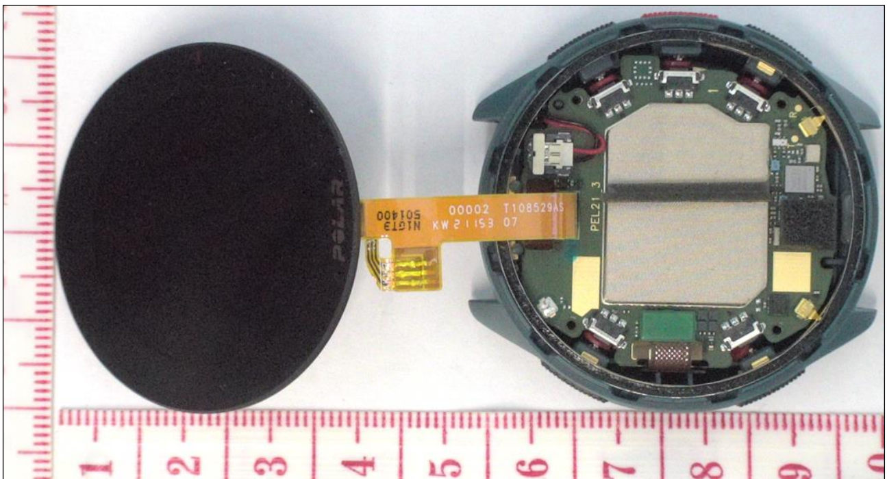
Figure 2. The display module separated.
