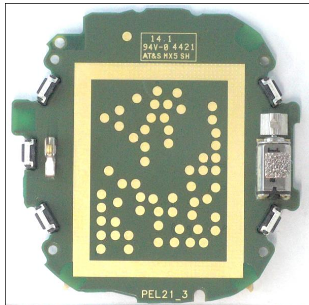
Figure 5. The main PWB from vibra motor side.
