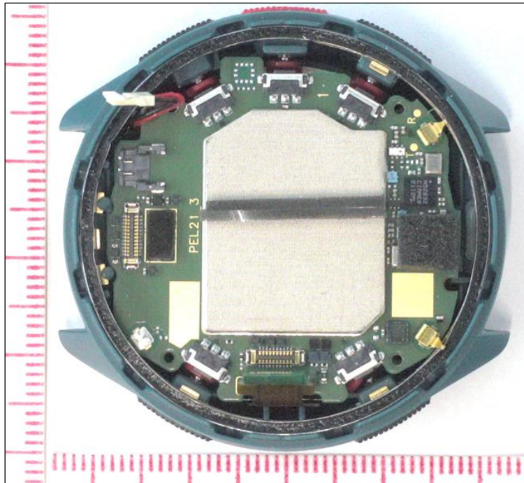
Figure 3. The connectors have been removed.
