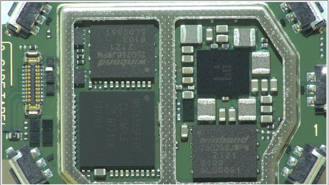
Figure 6. Component details 1.
