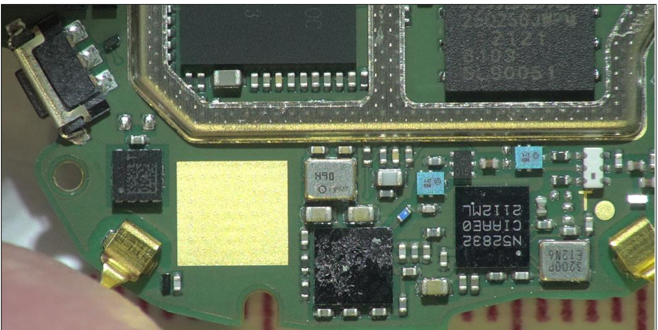
Figure 7. Component details 2.
