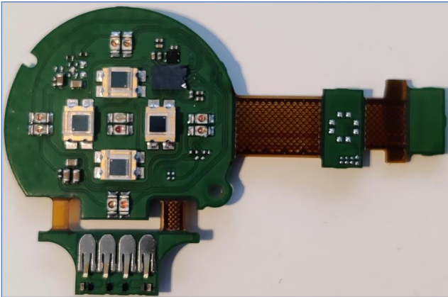
Figure 11. OHR PWB from component side.
