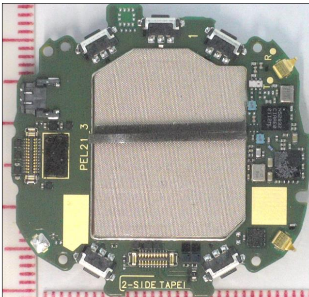
Figure 4. The main PWB from component side.
