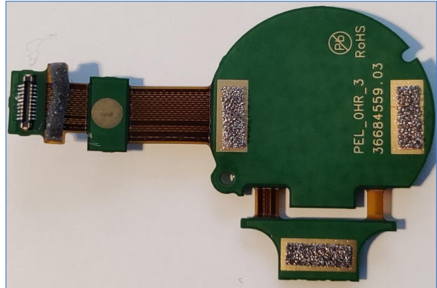
Figure 12. OHR PWB from other side.
