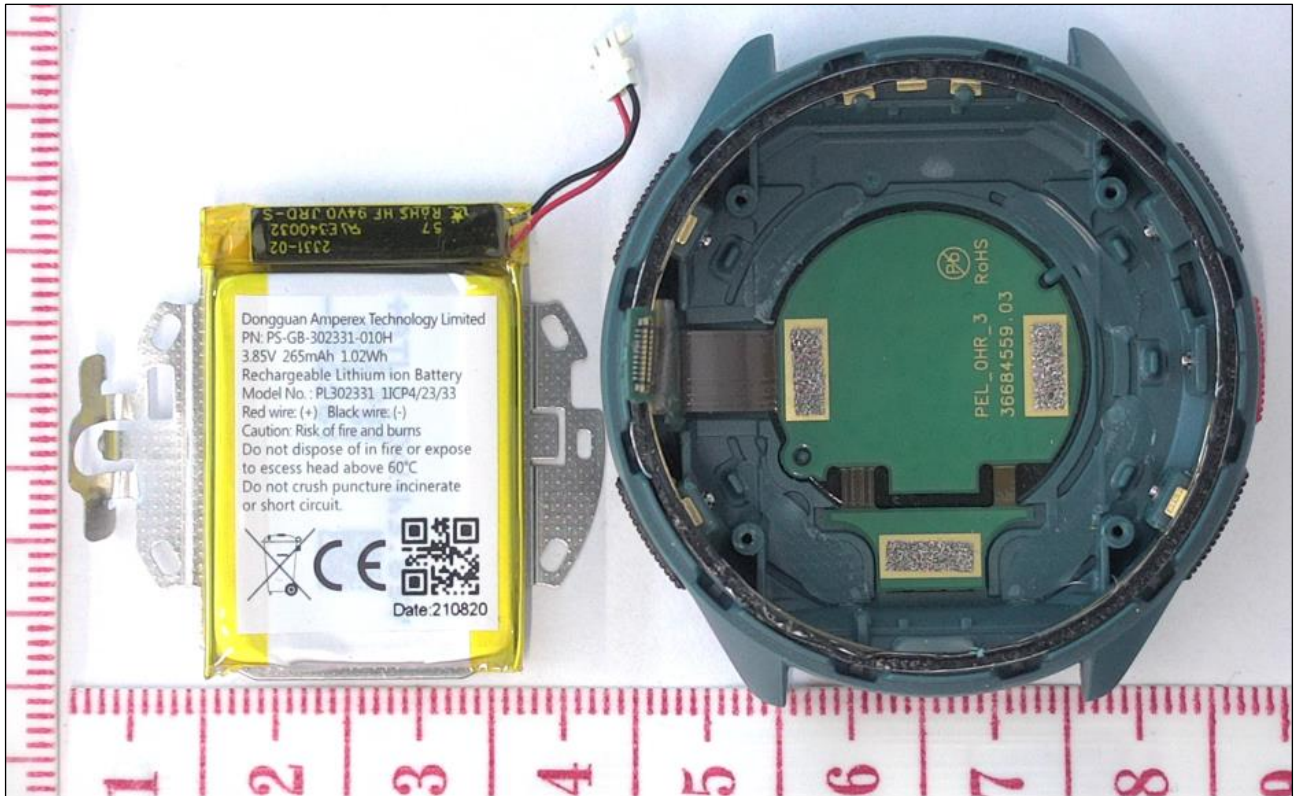
Figure 8. Battery removed.
