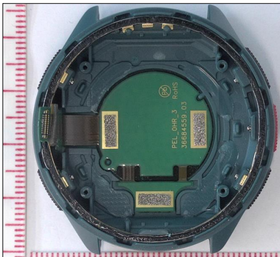
Figure 9. OHR PWB visible.
