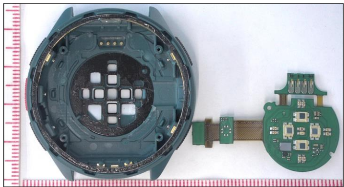
Figure 10. OHR PWB removed.
