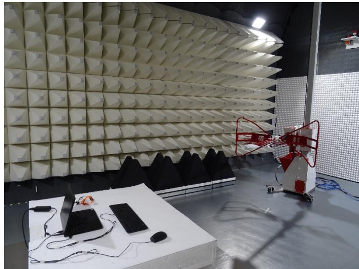
Radiated emission
