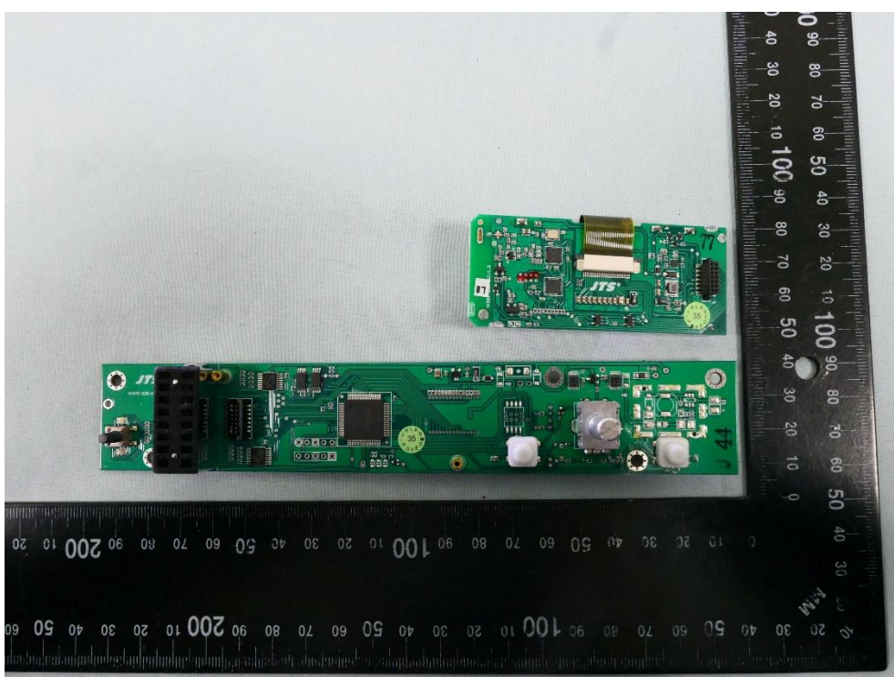
(42) EUT Photo
