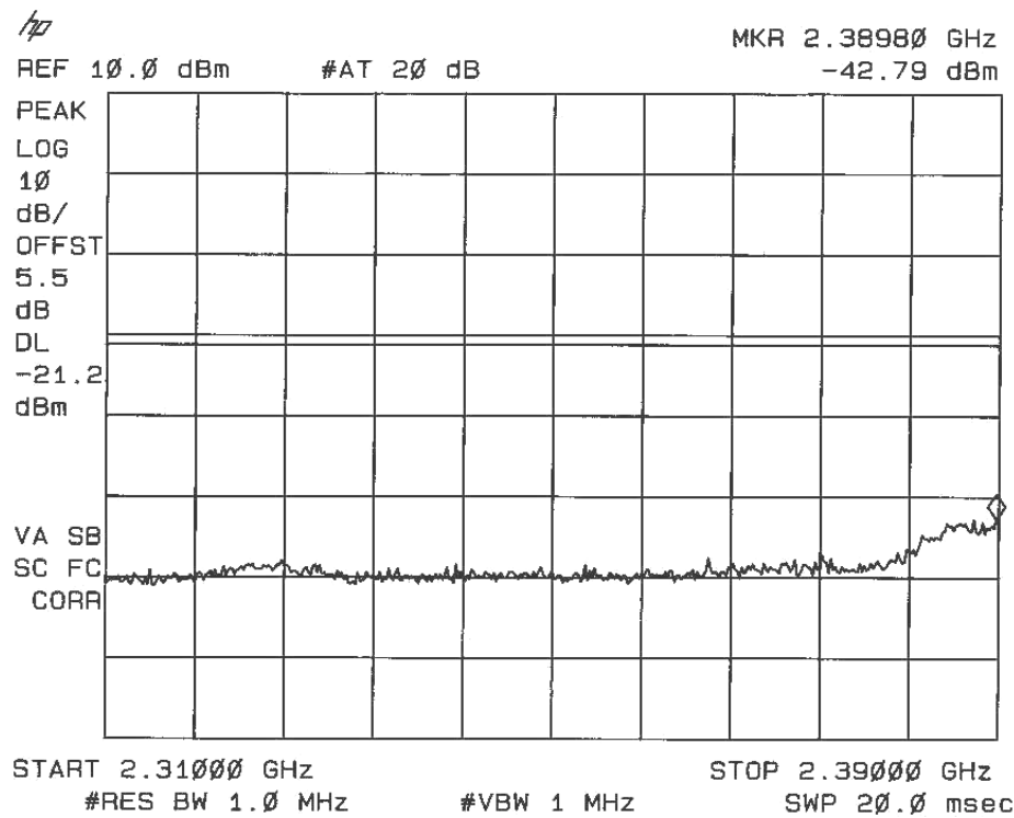
Figure 9.2: peak values in restricted band, All bitrate settings, conducted measurement, corrected for 2 dBi antenna gain and 2.6 dB cable losses. 74 dBµV/m :: -21.2 dBm display line setting.
