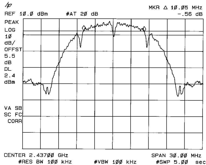
Figure 9.6: minimum 6 dB bandwidth at 2 Mbit/s.
