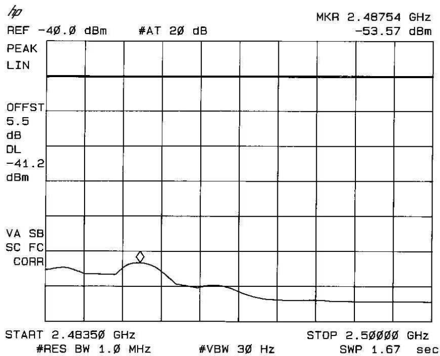
Figure 9.3: average values in restricted band, All bitrate settings, conducted measurement, corrected for 2 dBi antenna gain and 2.6 dB cable losses. 54 dBµV/m :: -41.2 dBm display line setting.
