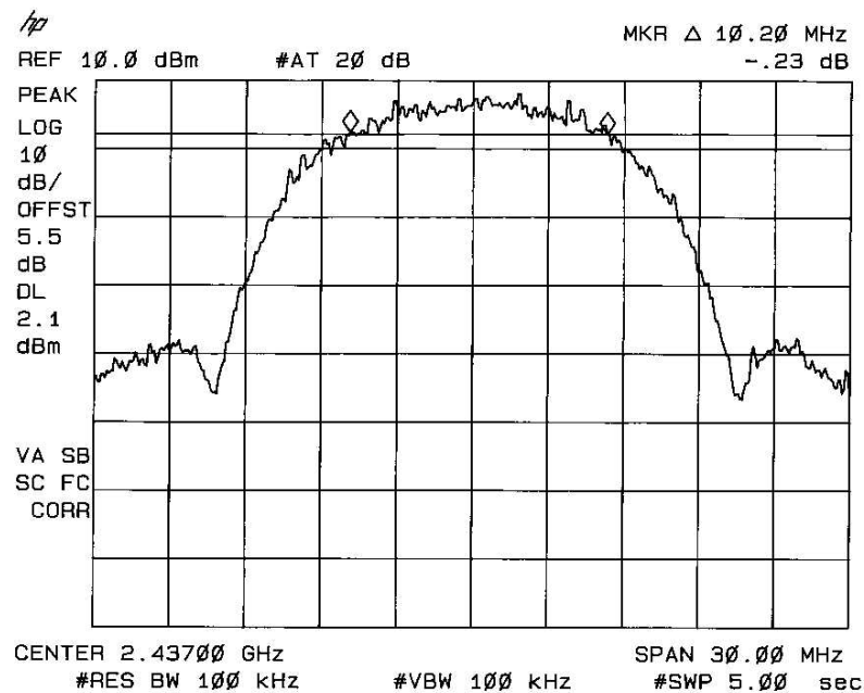
Figure 9.7: minimum 6 dB bandwidth at 5.5 Mbit/s.
