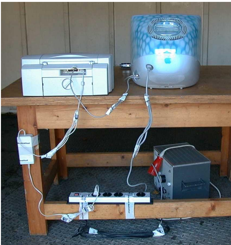
Figure 5.4: back picture of testconfiguration.
