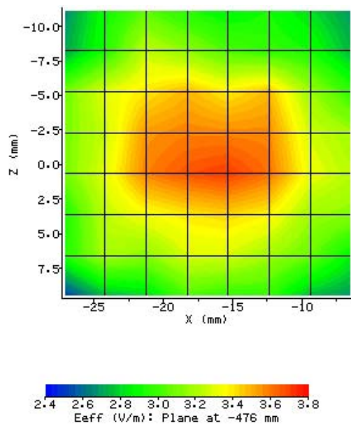
Figure 5: lapheld ch 164
