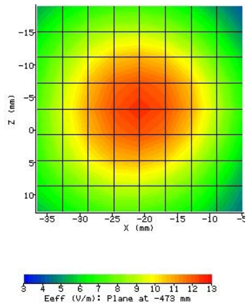
Figure 4: perpendicular ch 6
