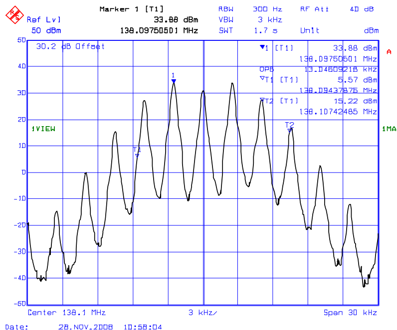
Plot 5.9.4.1.1(ii) 99% Occupied Bandwidth Carrier Frequency: 138.1 MHz; Channel Spacing: 25 kHz; Power: 10 W Modulation: FM with 2.5 KHz sine wave signal
