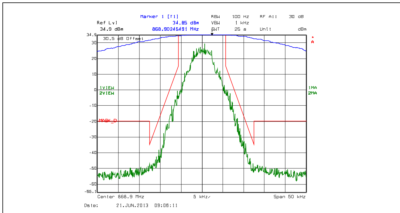
Plot 5.4.4.2.83. Emission Mask D, 12.5 kHz Channel Spacing, F1D, High Power, 868.9 MHz
