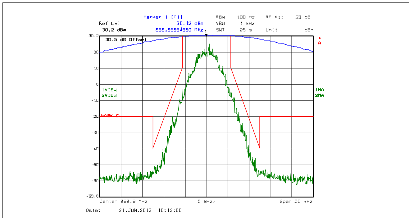
Plot 5.4.4.2.84. Emission Mask D, 12.5 kHz Channel Spacing, F1D, Low Power, 868.9 MHz
