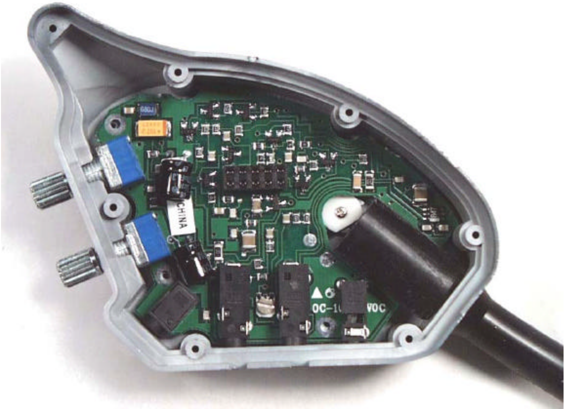
radio
