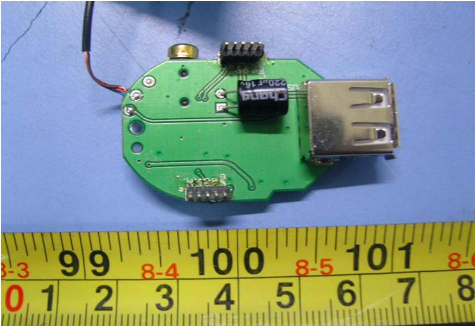
11.6PCB2 - Back View
