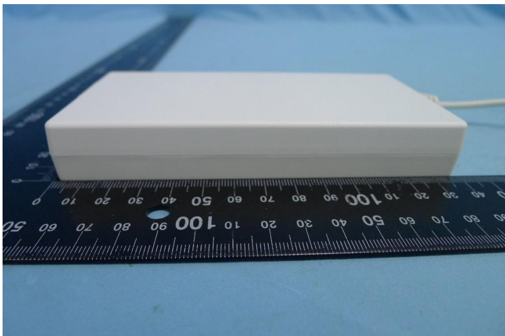
(12) EUT Photo(Adapter)
