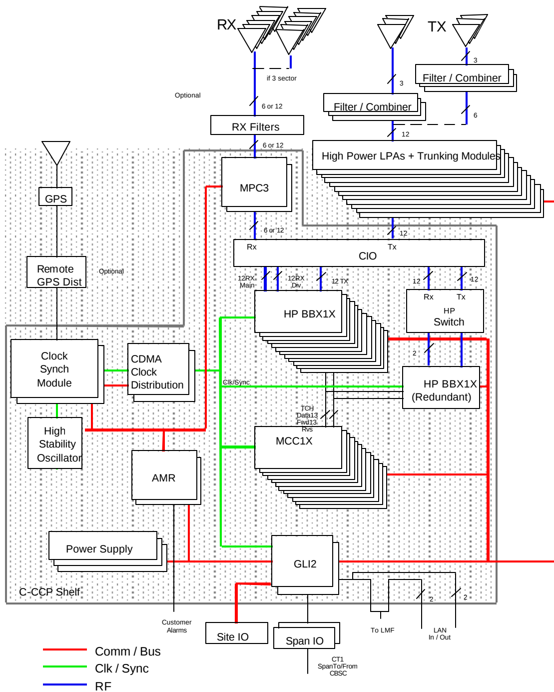
-48V SC 4812T @ 800 MHz CDMA BTS Frame Block Diagram
