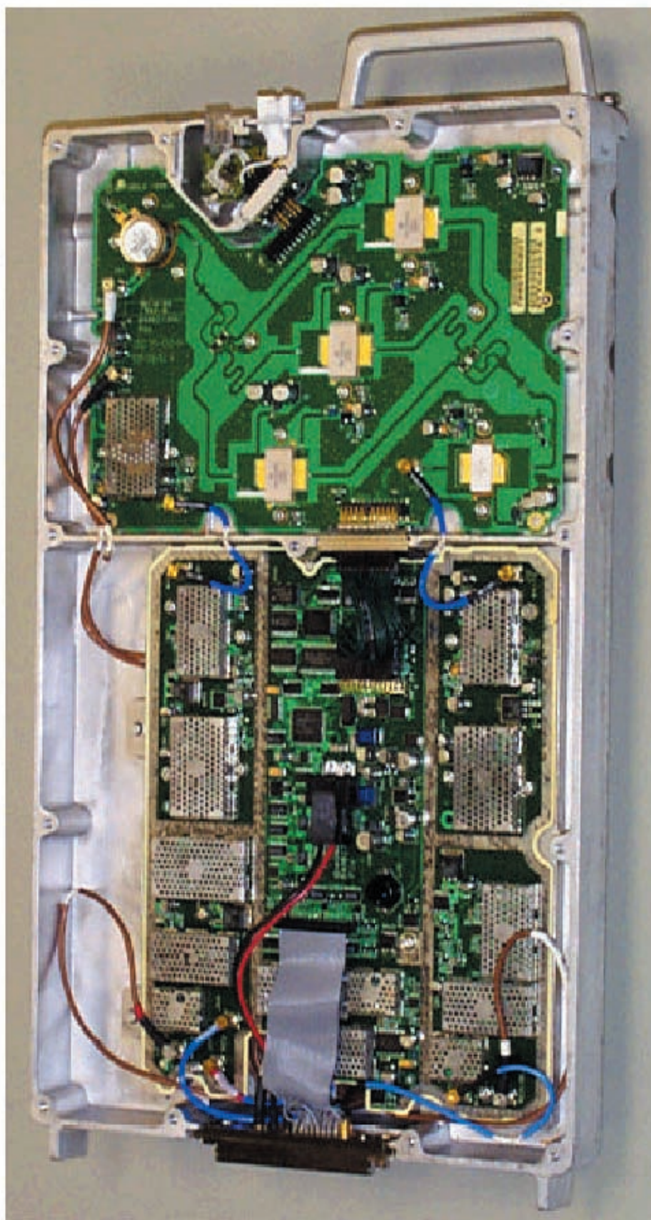
IHET5AP2 SC4812ETL 800MHz LPA without Cover
