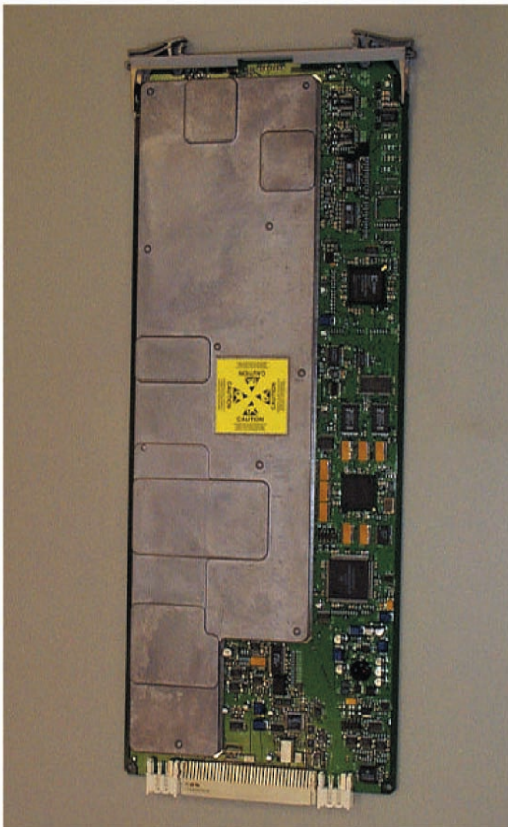
IHET5AP2 SC4812ETL 800 MHz BBX2 With Cover
