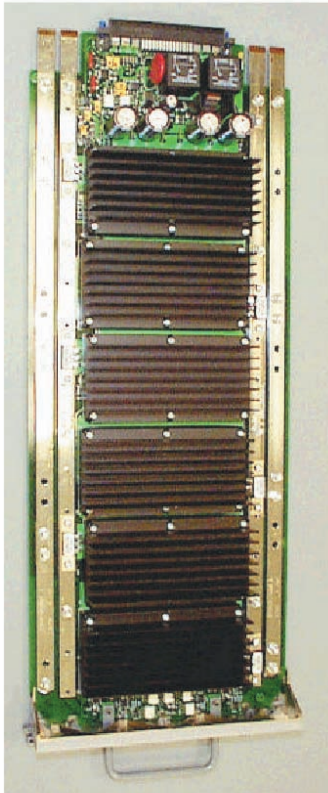
IHET5AP2 4812ETL 800 MHz Power Supply Front
