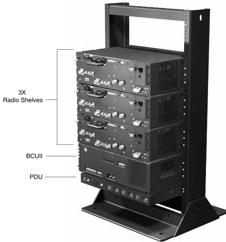
Figure 3-1 Indoor system
