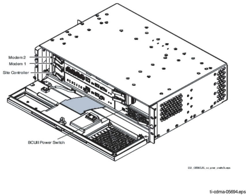
Figure 3-6 BCUII physical design
