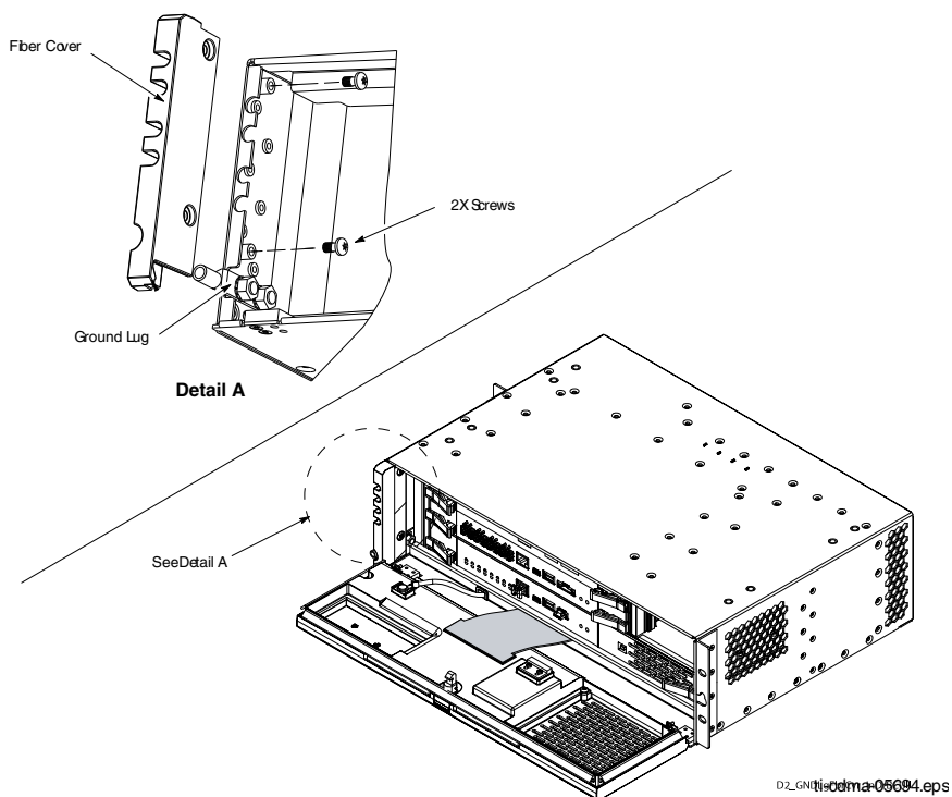
Figure 8-4 BCUII Fiber Cover
