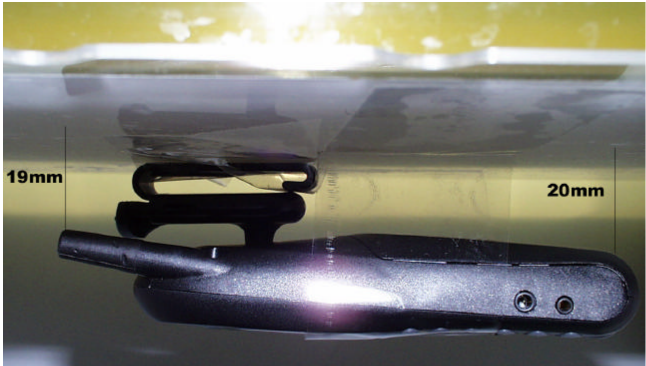
Figure 4. Phone In Supplied Belt Clip Against Phantom
