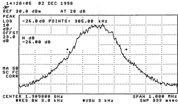
Figure 8.6: Channel 810, -26dBc Bandwidth
