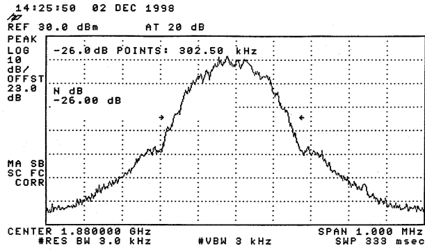
Figure 8.5: Channel 661, -26dBc Bandwidth
