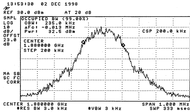
Figure 8.2: Channel 661, 99% Power Bandwidth
