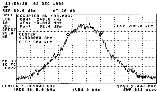
Figure 8.3: Channel 810, 99% Power Bandwidth
