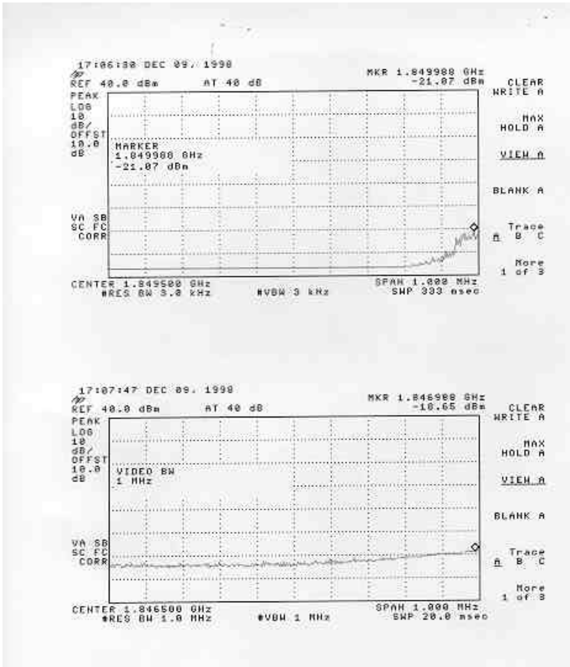
(UPPER) Figure 9.1: Carrier 1850.2 MHz, Spectrum 1849 to 1850 MHz, RBW/VBW = 3 kHz.
