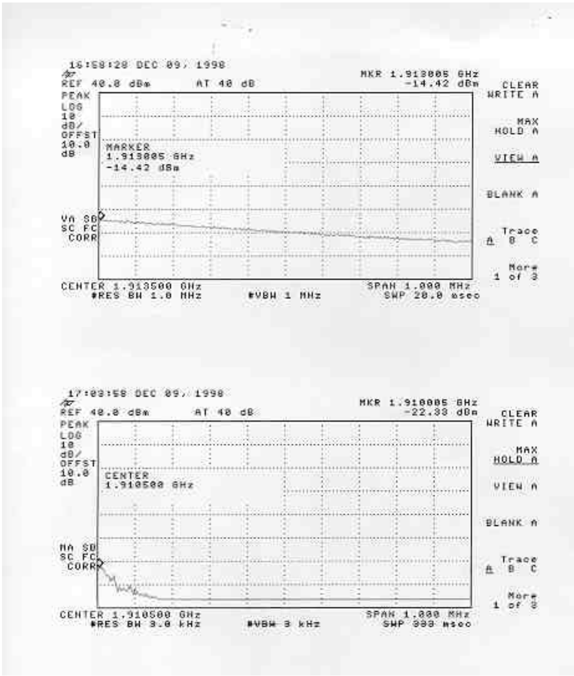
(UPPER) Figure 9.3: Carrier 1909.8 MHz, Spectrum 1913 to 1914 MHz, RBW/VBW = 1 MHz.
