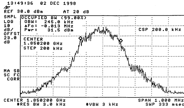
Figure 8.1: Channel 512, 99% Power Bandwidth
