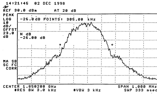
Figure 8.4: Channel 512, -26dBc Bandwidth
