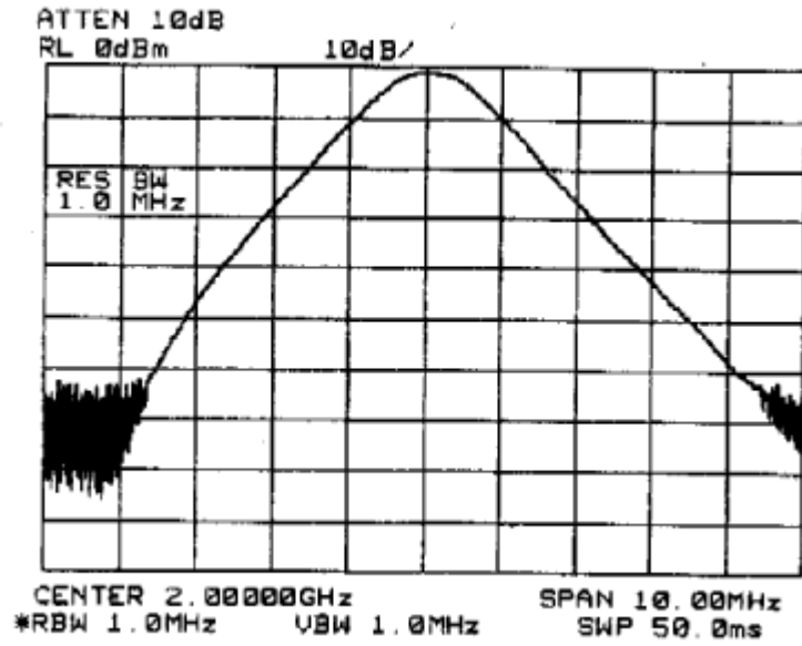
Figure 9.5: Spectrum Analyzer 1 MHz Resolution Bandwidth Filter Response.
