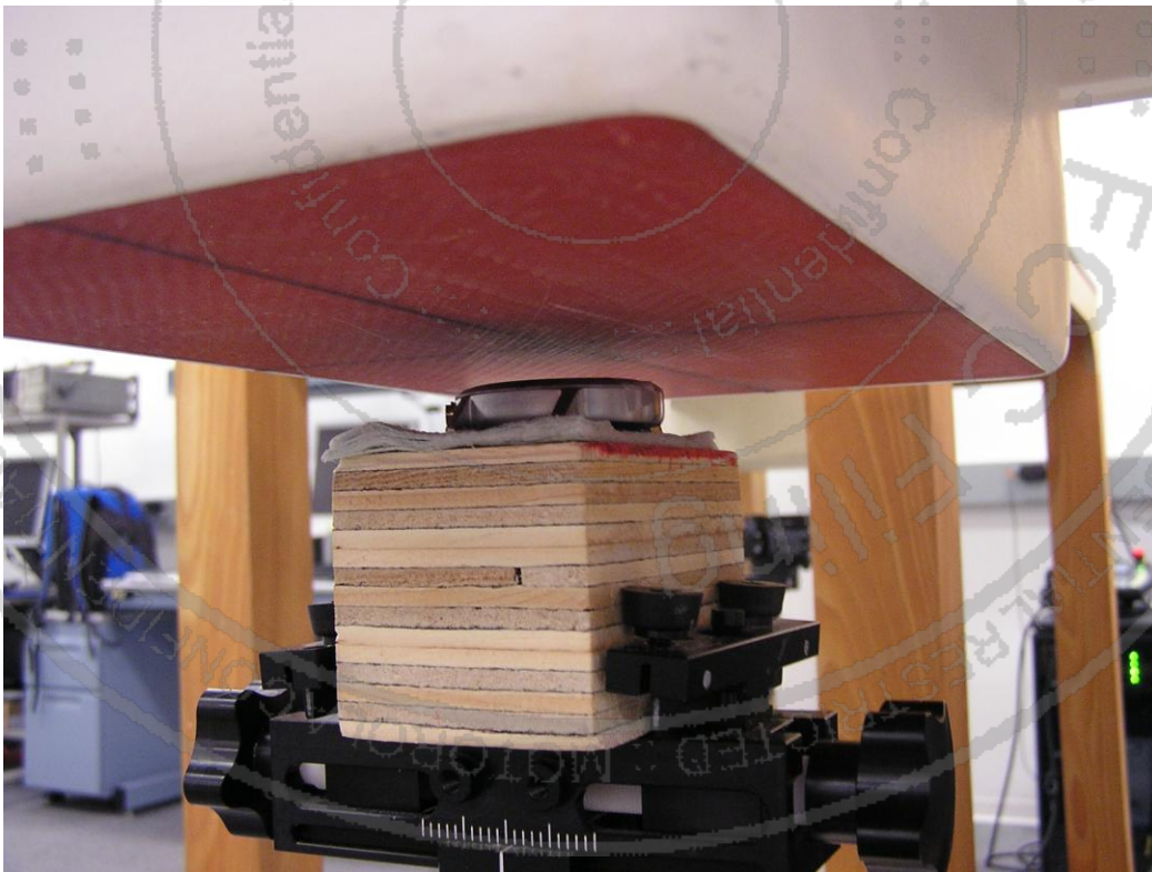
Figure 12: Front of Large Body Device (without band) against Phantom
