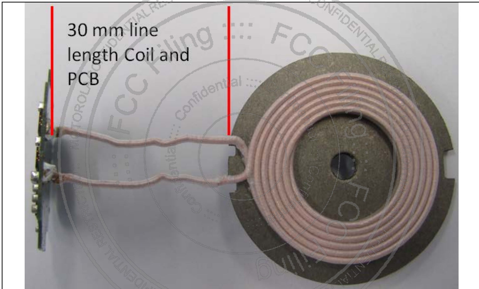
Photograph 9-5: Coil / PC Board Connection.
