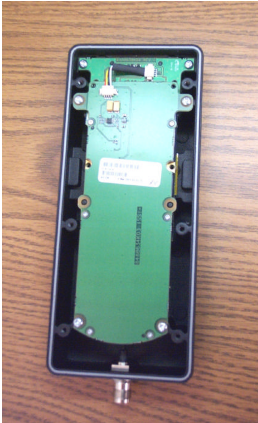
Figure 9.0-5 Audio Interface Board - Bottom Side
