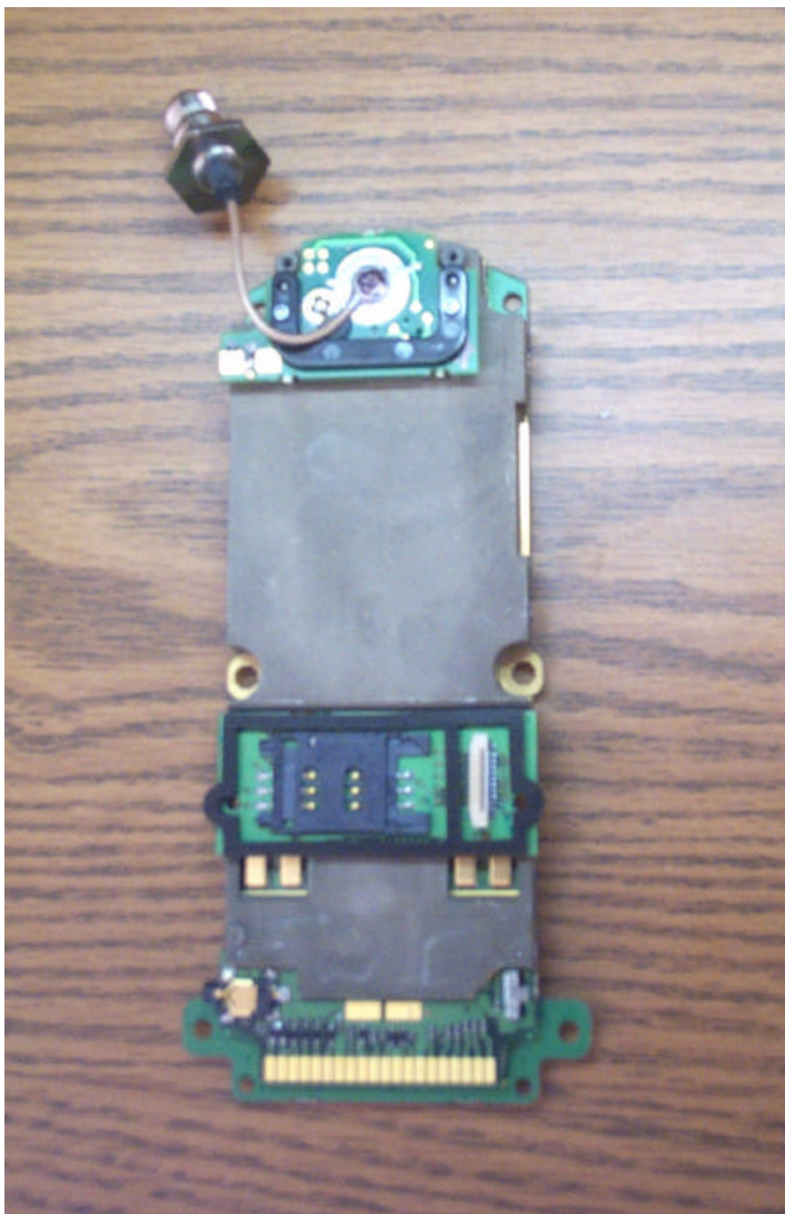
Figure 9.0-2 Transceiver Board - Top Side with Shields
