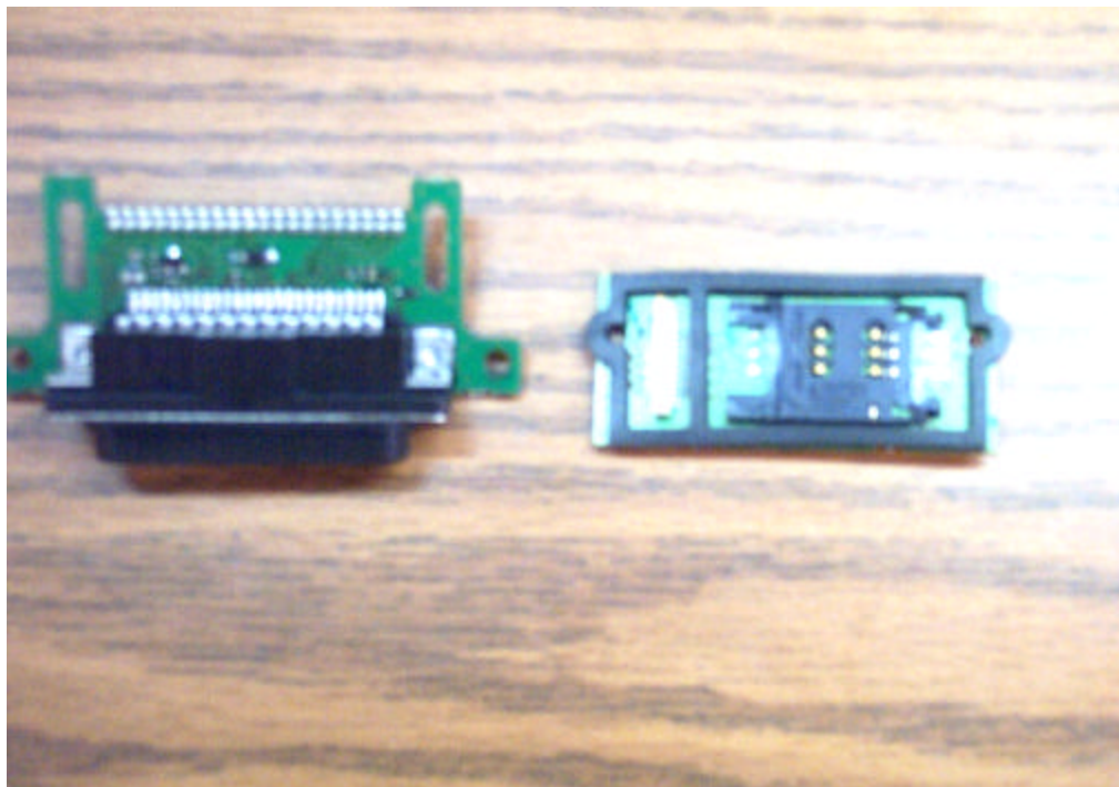
Figure 9.0-8 Top Side of Accessory Interface Board & SIM Interface Board
