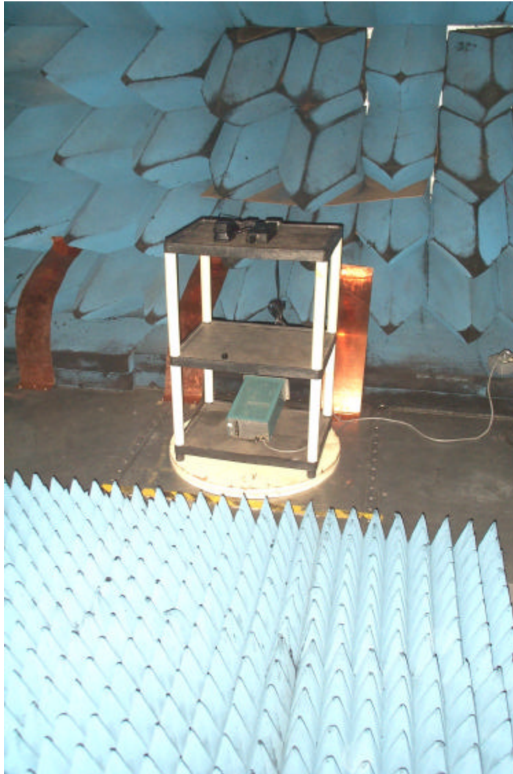
Figure 7.0-3 Radiated Emissions Test Setup - Harmonics
