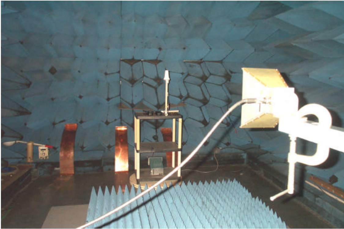
Figure 7.0-4 Radiated Emissions - Harmonics
