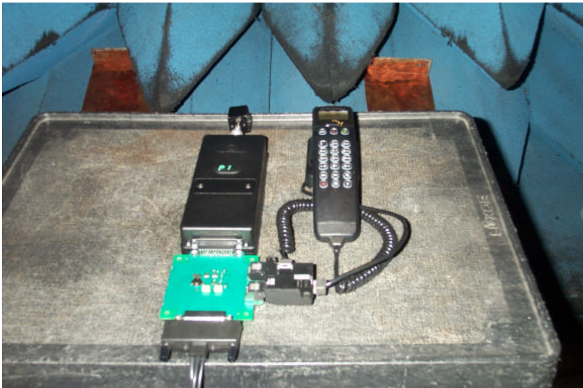
Figure 7.0-1 Radiated Emissions Test Setup – Prescans & Harmonics
