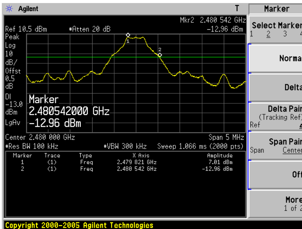
Channel 78 (2480MHz)
