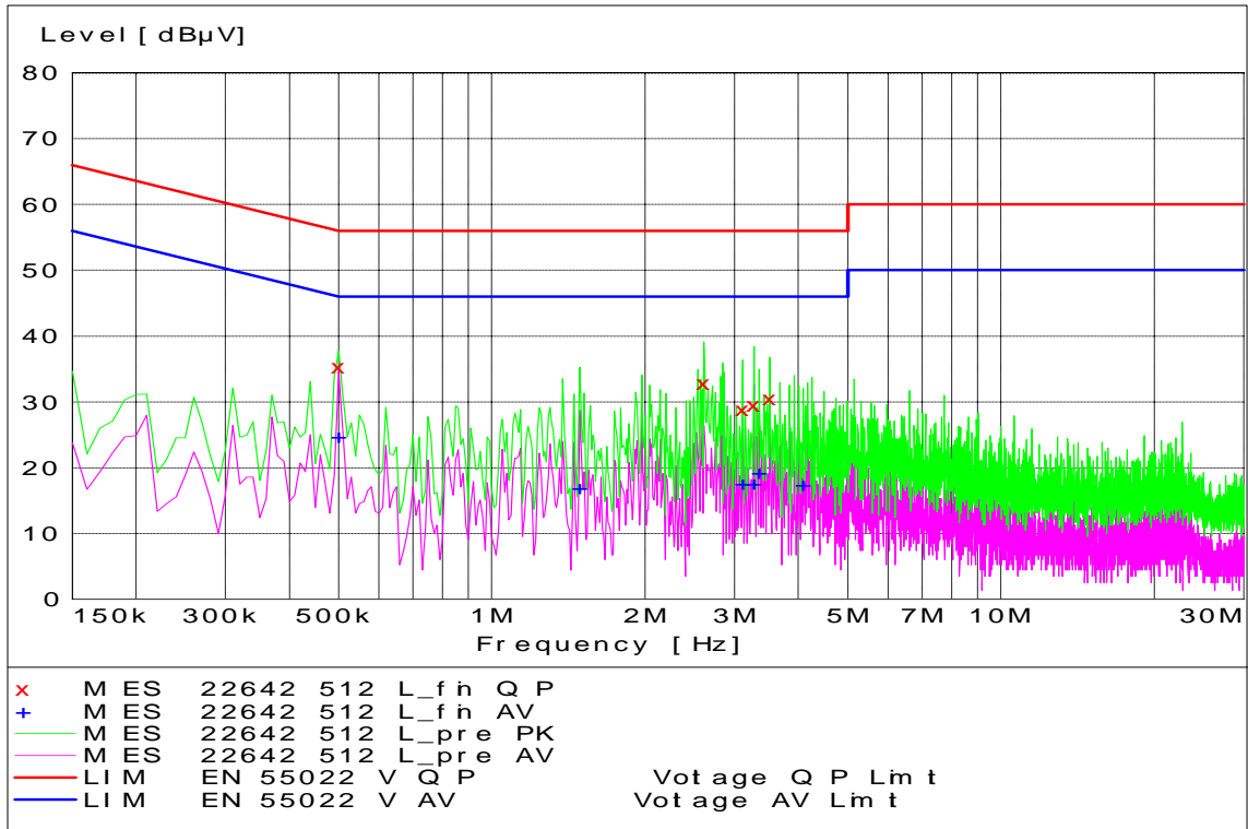
GSM 1900 Channel 512 - Tx Mode - Line Coupling
