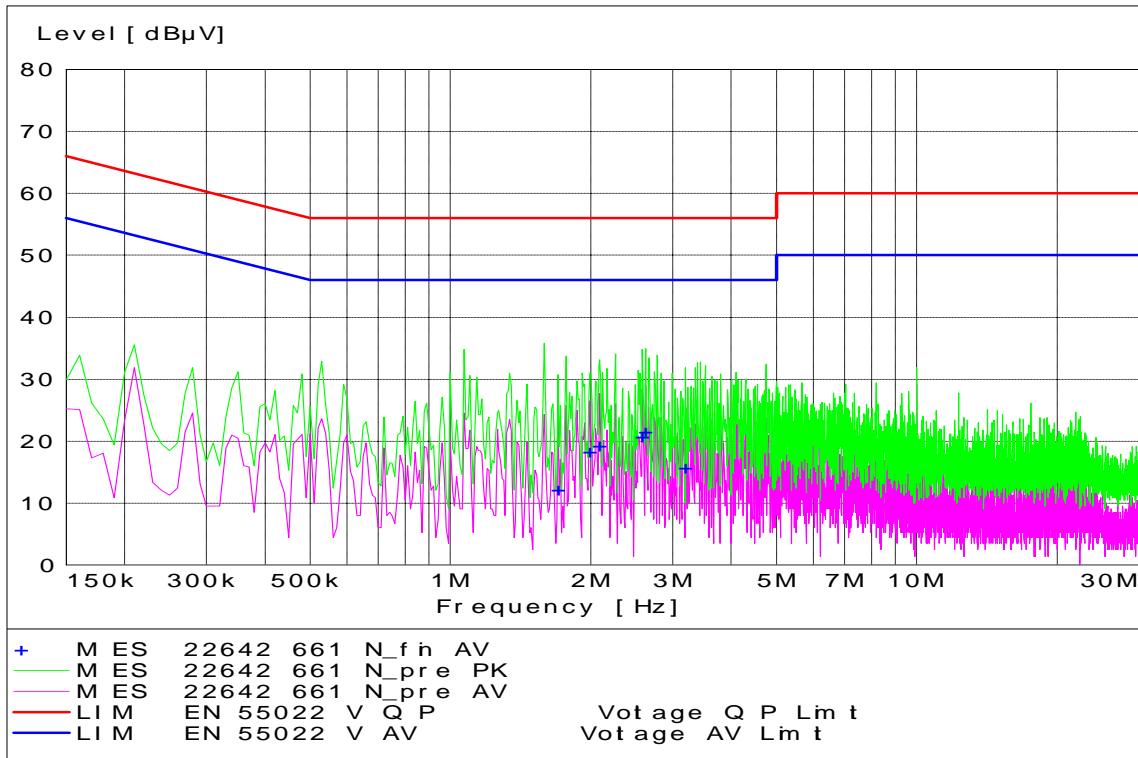
GSM 1900 Channel 661 - Tx Mode - Neutral Coupling
