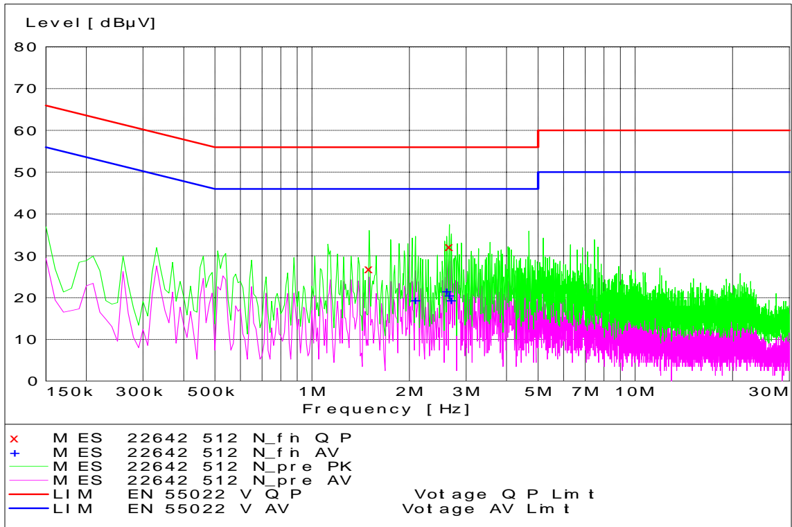
GSM 1900 Channel 512 - Tx Mode - Neutral Coupling
