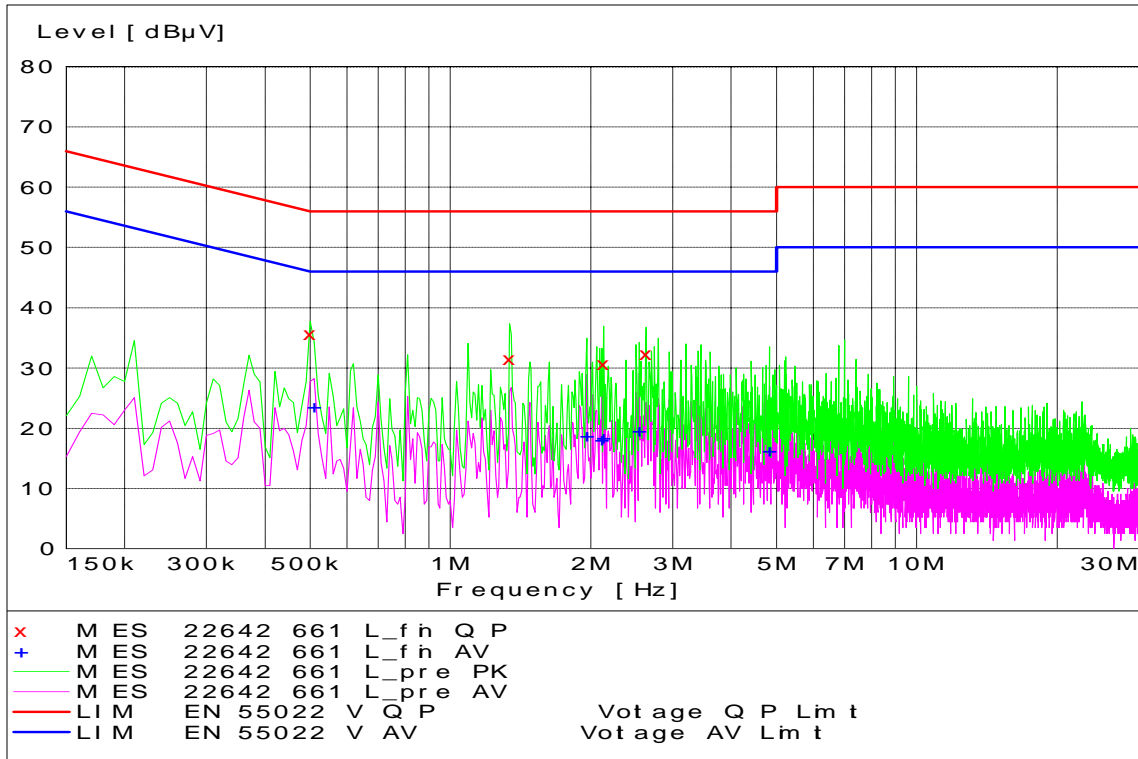
GSM 1900 Channel 661 - Tx Mode - Line Coupling
