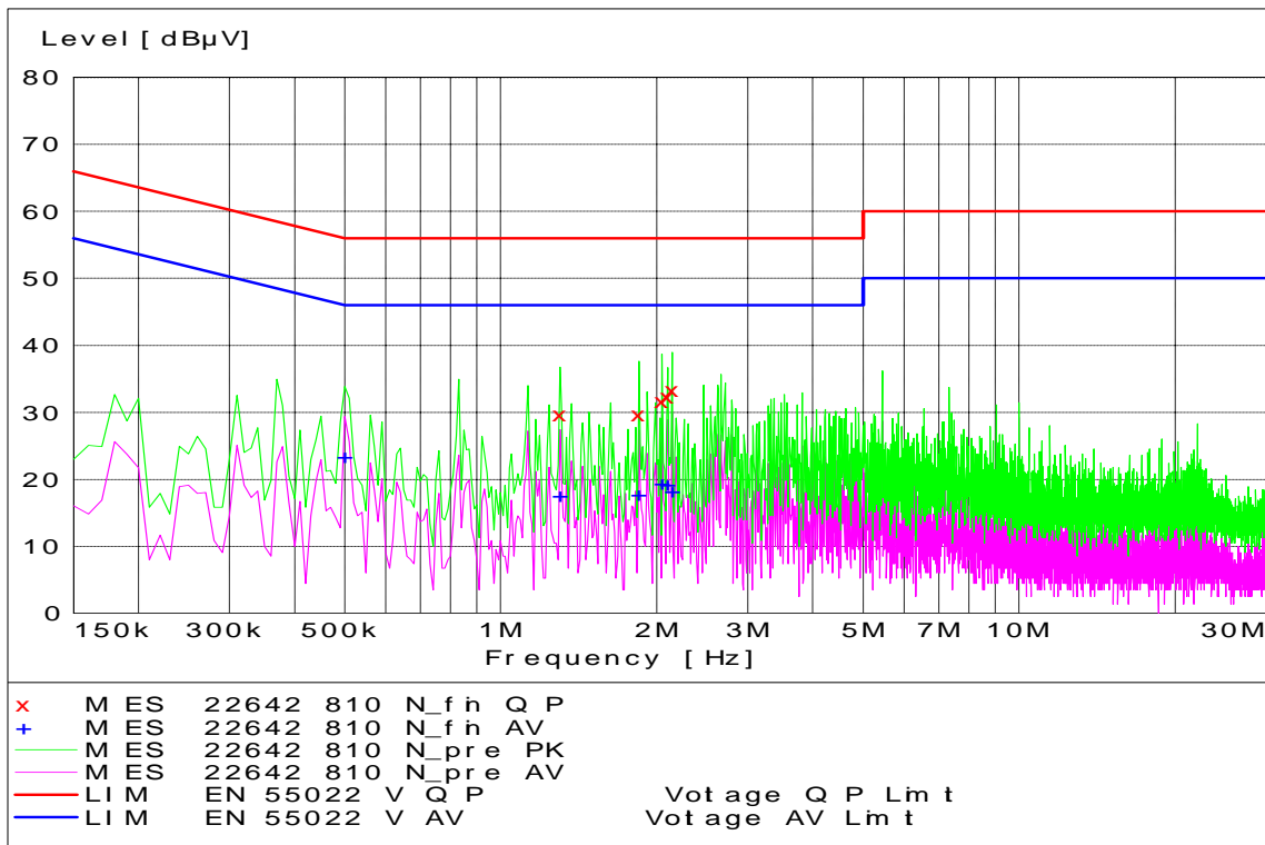
GSM 1900 Channel 810 - Tx Mode - Neutral Coupling
