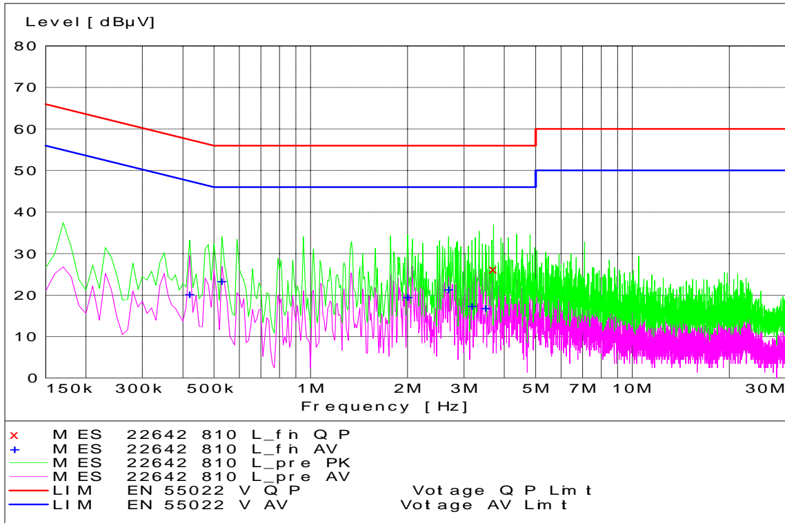
GSM 1900 Channel 810 - Tx Mode - Line Coupling
