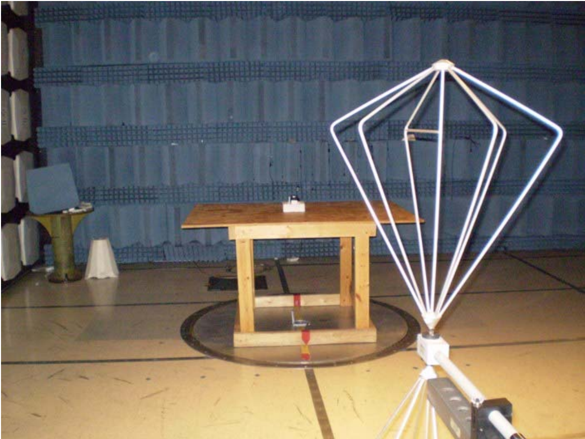
EMC Report #21534 Tx Radiated
