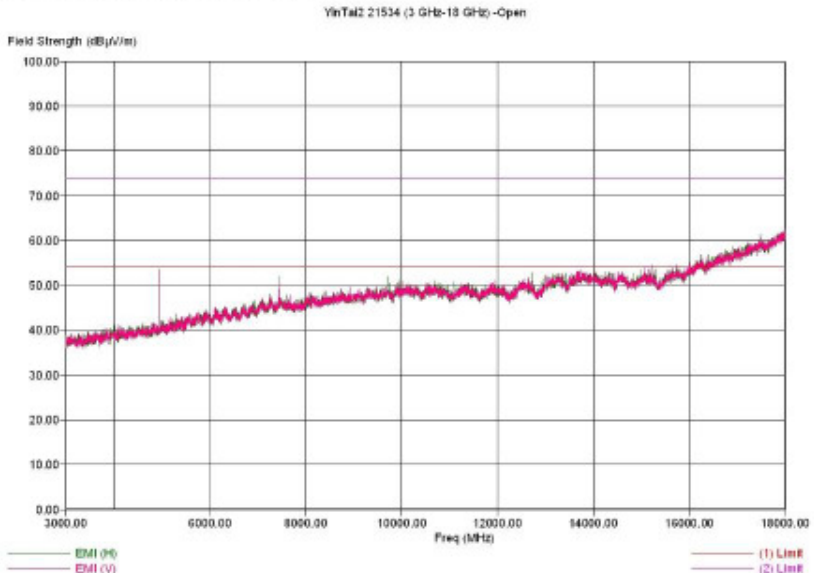
3-18 GHz High Channel Dual Polarization Z
