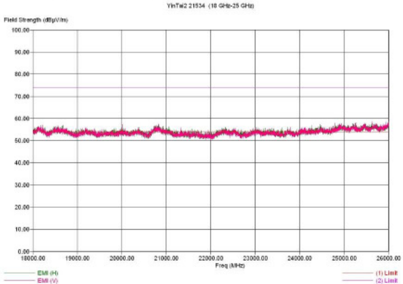
18-25 GHz Low Channel Dual Polarization Y
