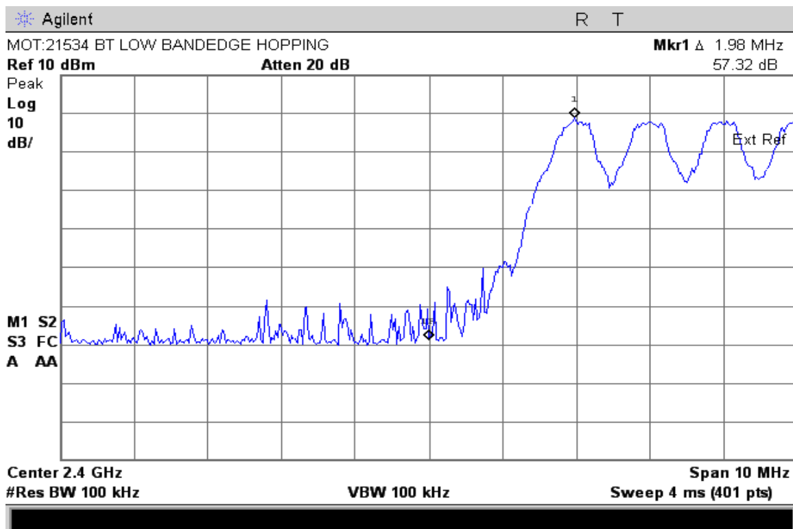
Non-EDR mode Low Bandedge with Hopping Enabled
