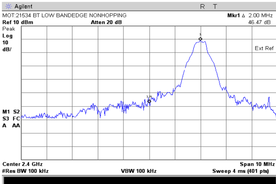
Non-EDR mode Low Bandedge with Hopping Disabled
