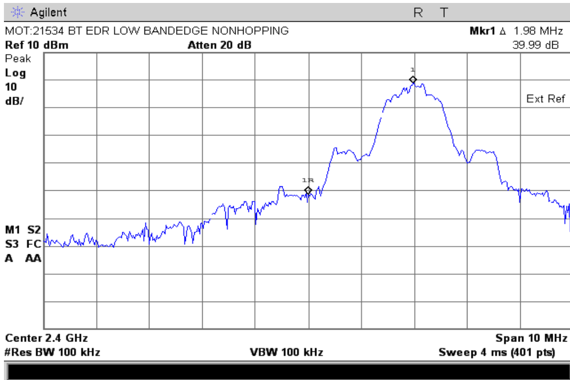
EDR mode Low Band Edge with Hopping Disabled
