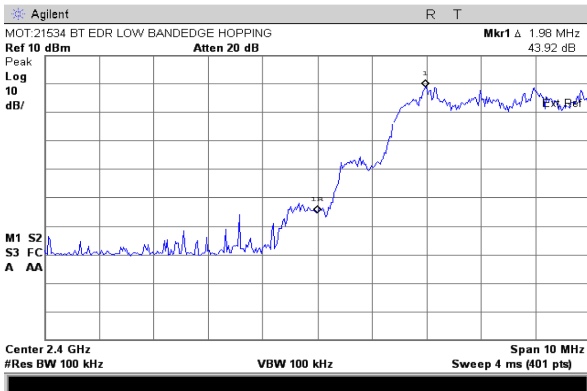
EDR mode Low Band Edge with Hopping Enabled
