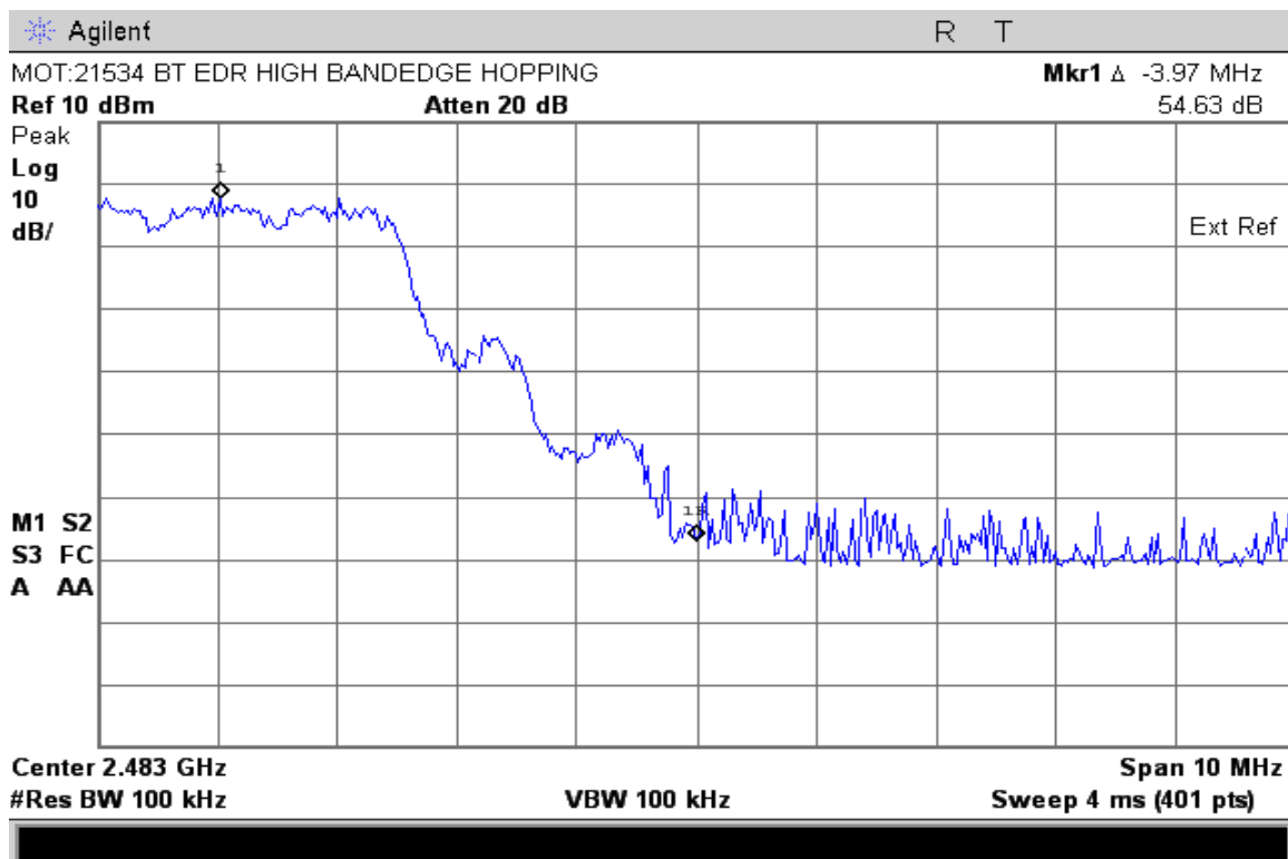
EDR mode High Band Edge with Hopping Enabled
