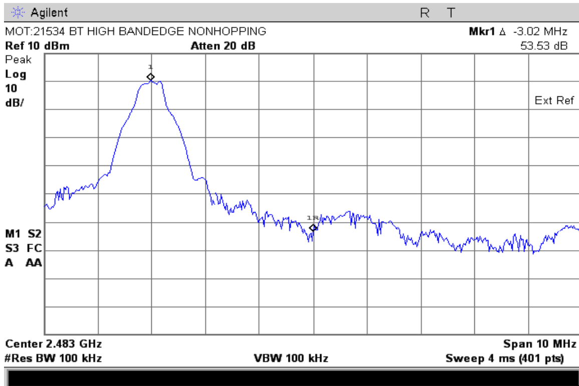
Non-EDR mode High Bandedge with Hopping Disabled
