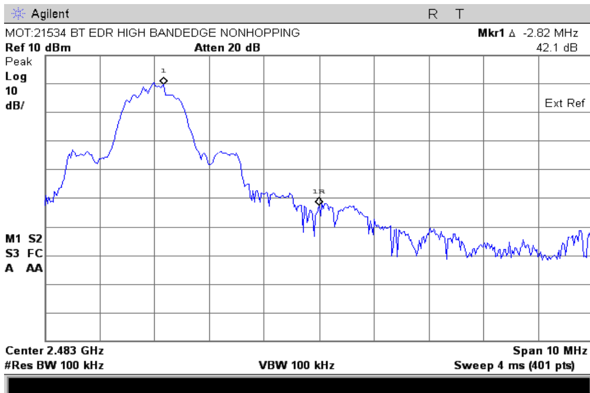
EDR mode High Band Edge with Hopping Disabled
