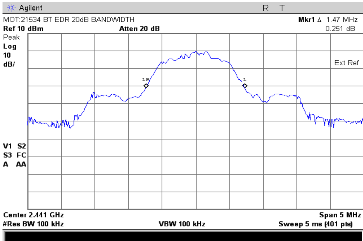
EDR mode 20dB Bandwidth
