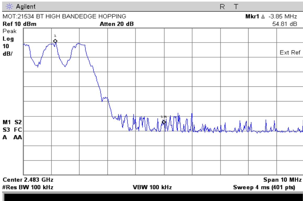
Non-EDR mode High Bandedge with Hopping Enabled
