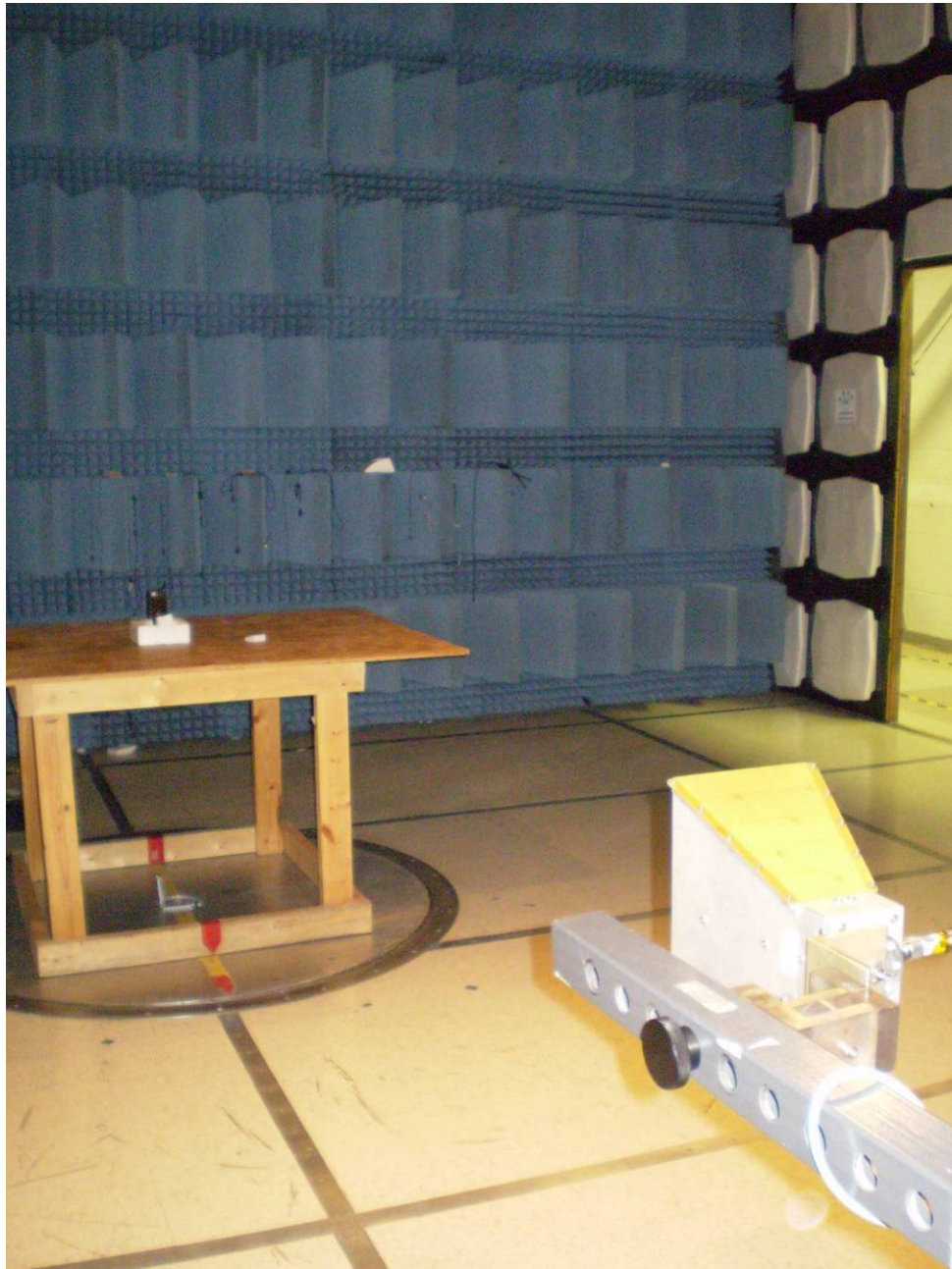
Radiated Emissions
