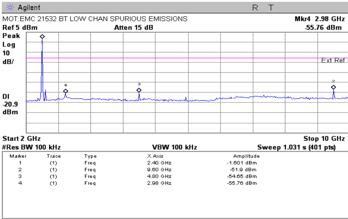
Conducted Spurious Emissions 2-10GHz (Low Channel Enabled)
