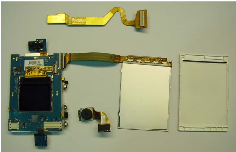
LCD Module & CLi Module & Flip RFPC Board & Hinge FPC Board & VGA Camera & 2M-Pixel Camera & Receiver Speaker
