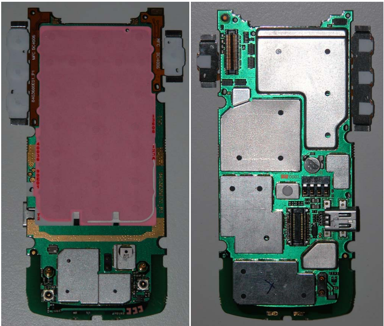
MAIN PCB – Front and Rear Views
