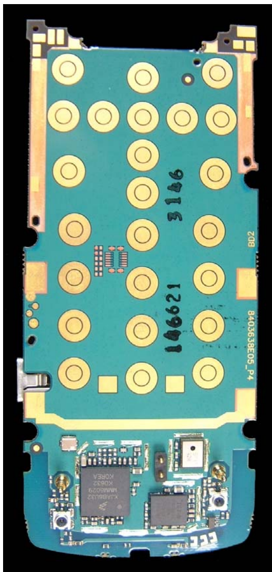
MAIN PCB – Front and Rear Views – without shields
