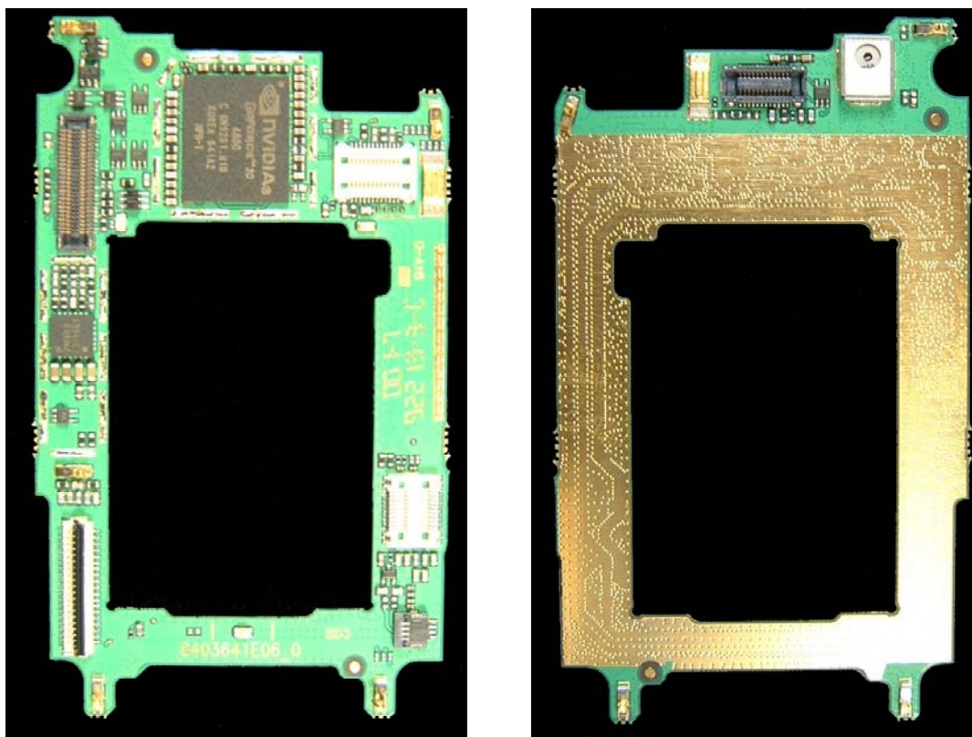
FLIP PCB – Front and Rear views – without shields
