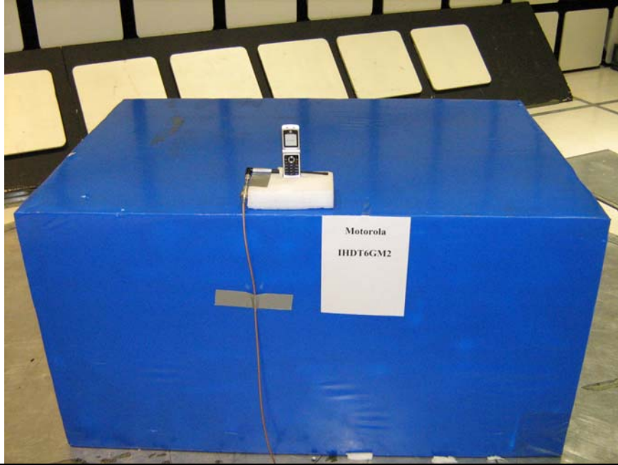
Figure 1 Test setup for Radiated Emissions
