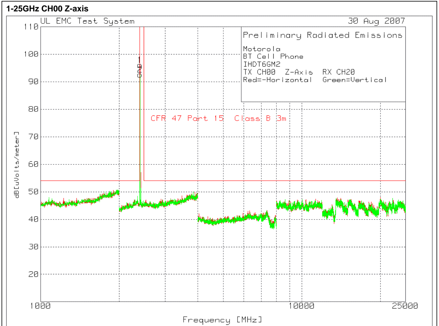
Figure 13 Radiated Emissions Graph
