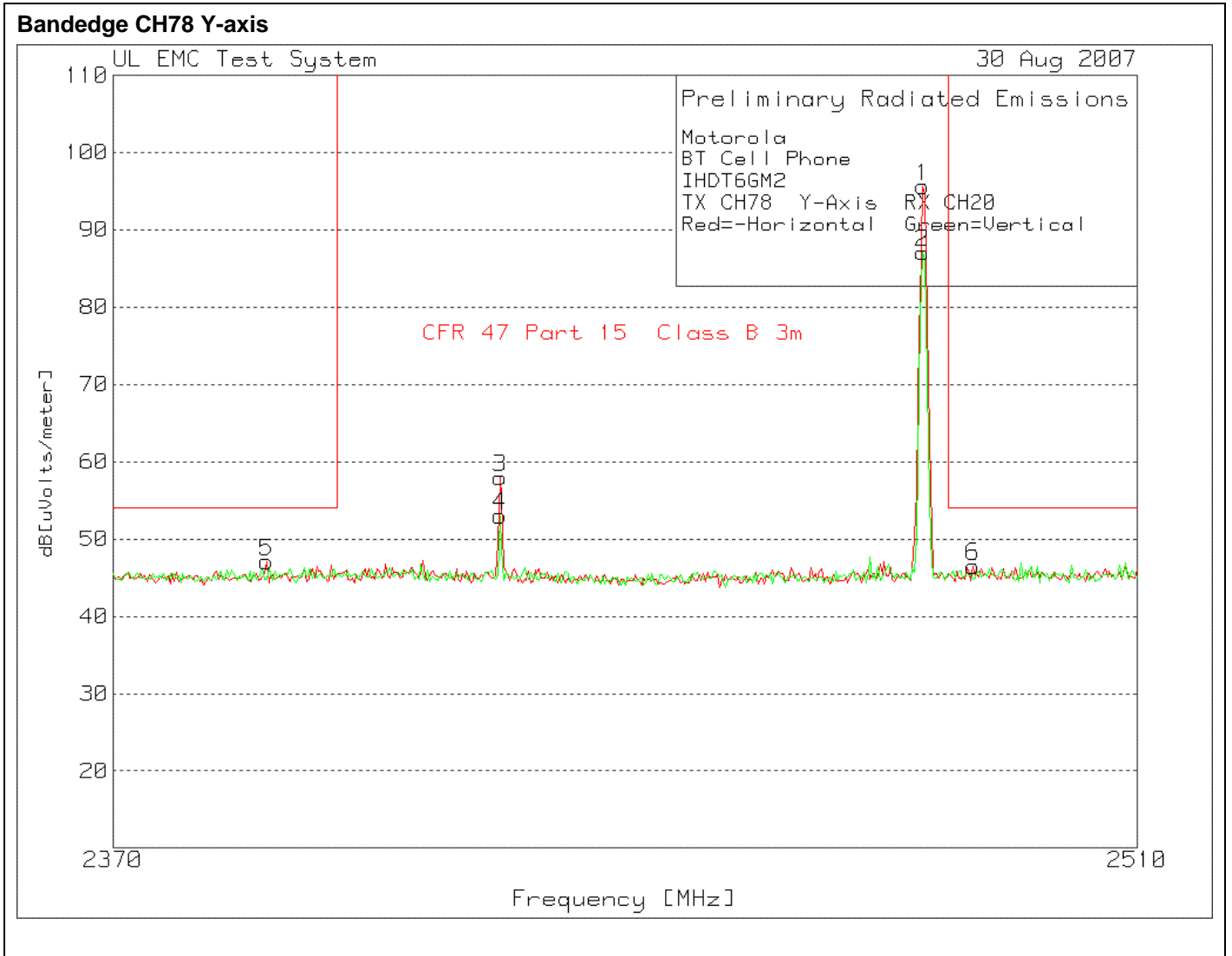
Figure 24 Radiated Emissions Graph
