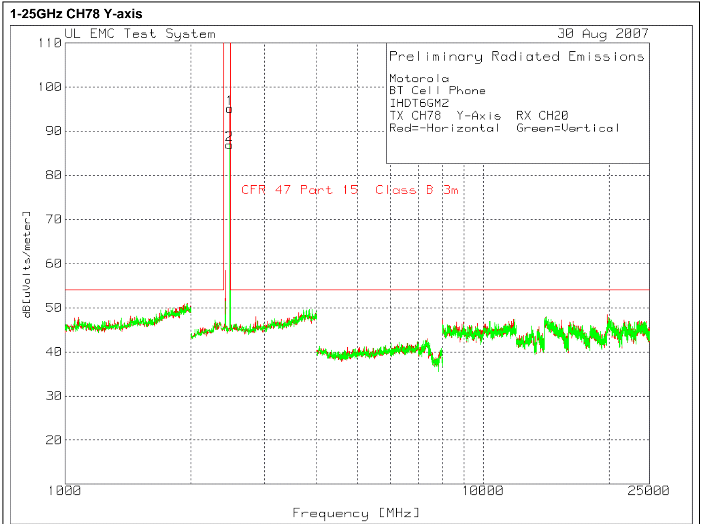
Figure 18 Radiated Emissions Graph
