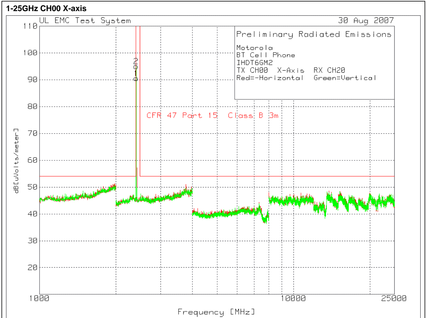
Figure 11 Radiated Emissions Graph
