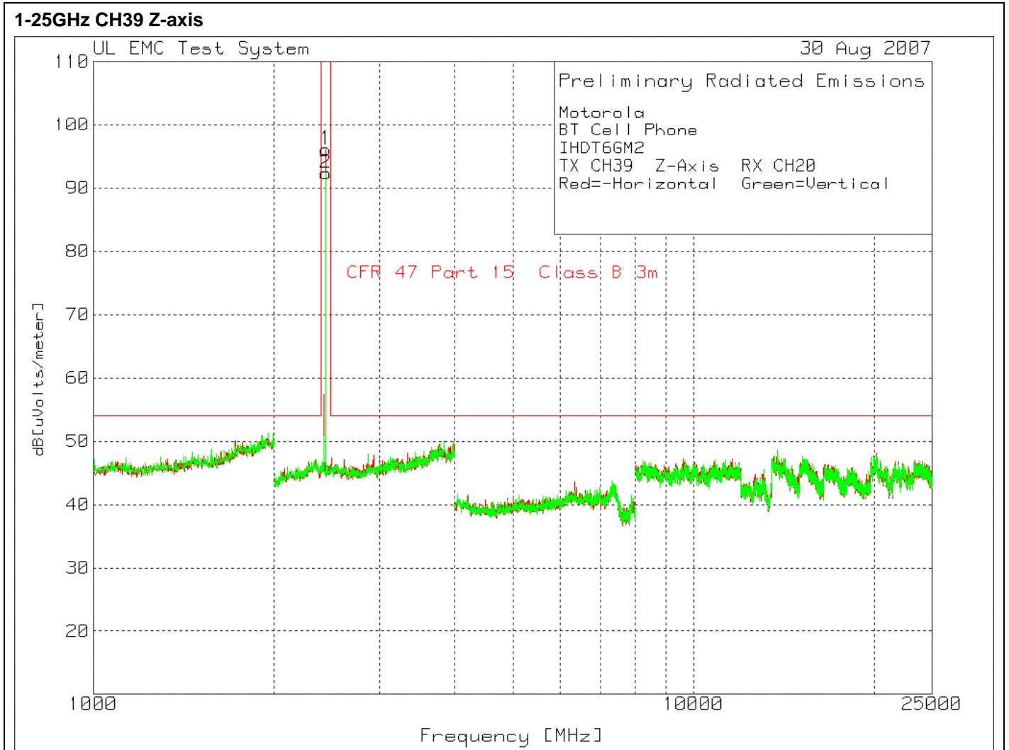
Figure 16 Radiated Emissions Graph
