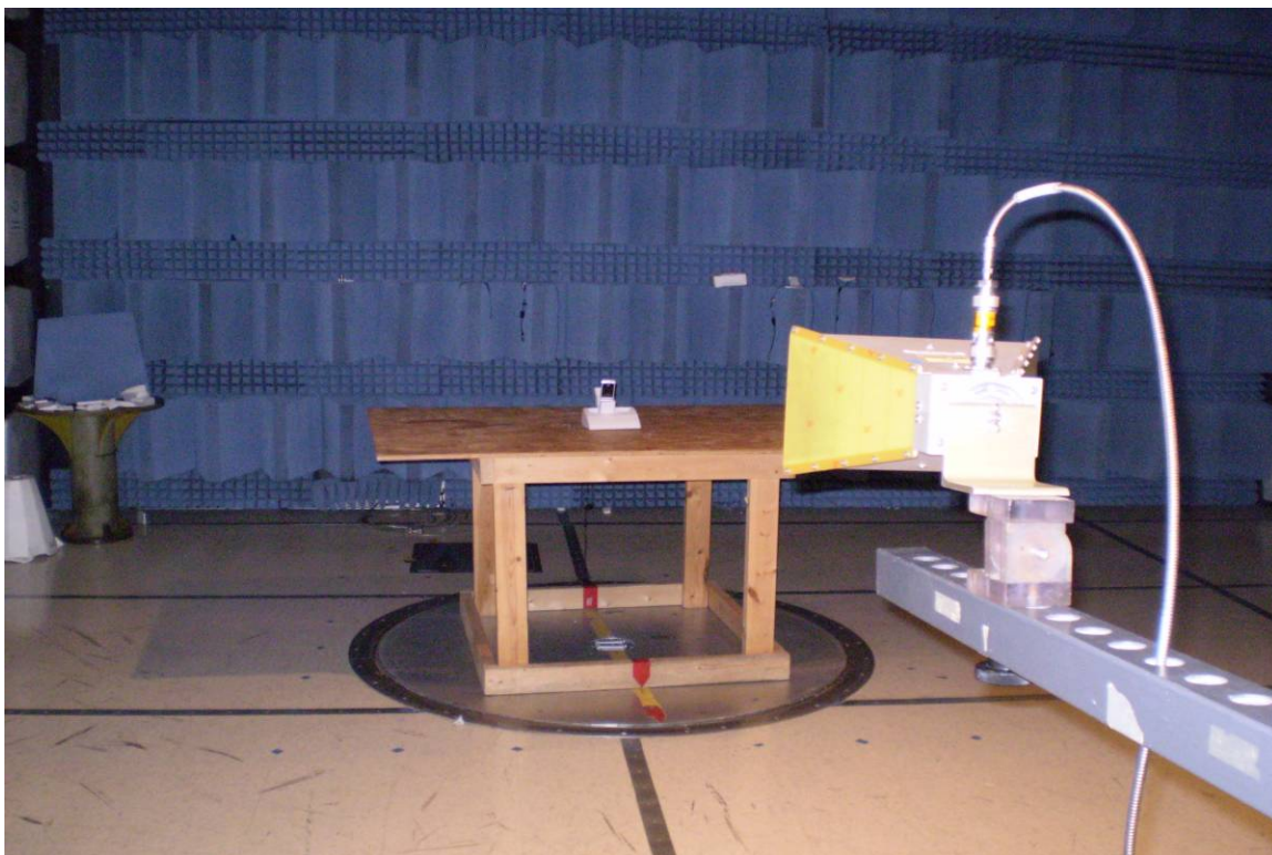
Tx Radiated
