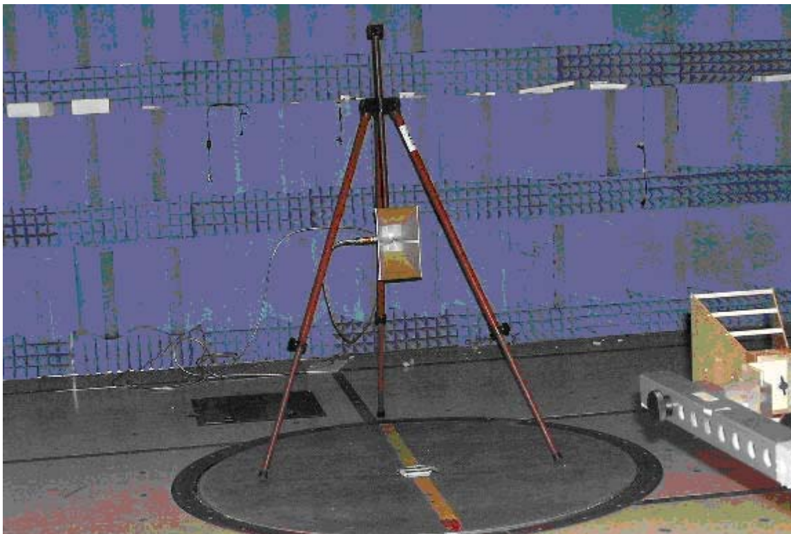
Antenna Substitution
