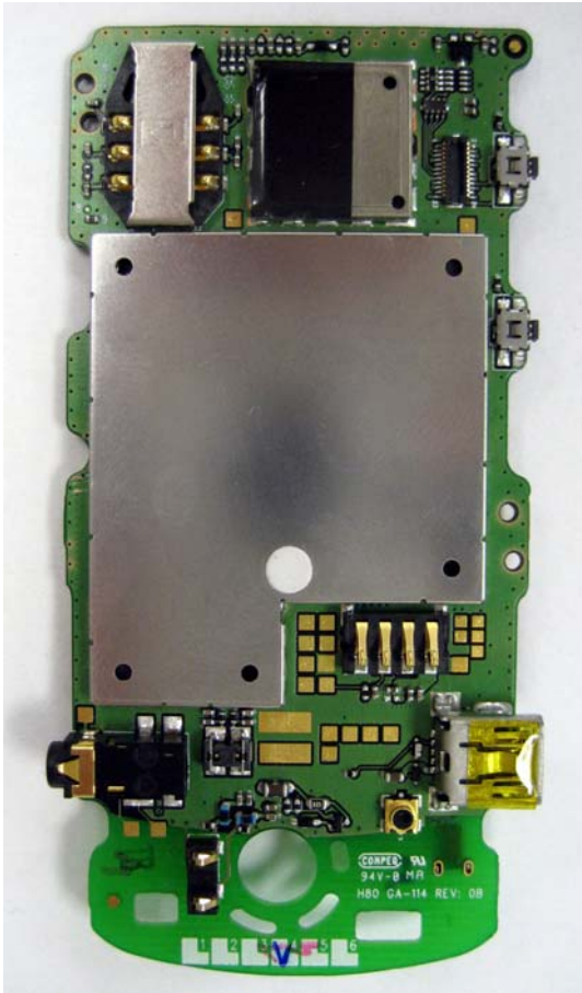
Main Board Bottom With Shields
