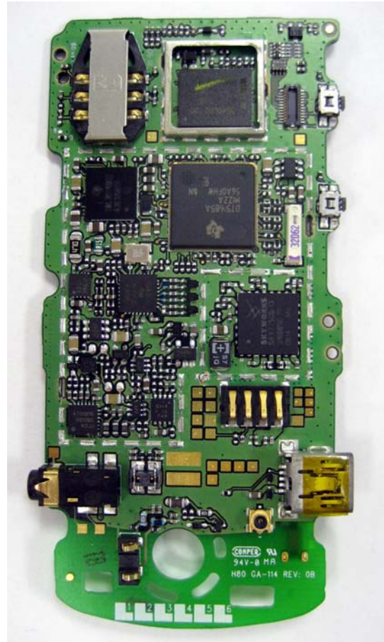
Main Board Bottom Without Shields
