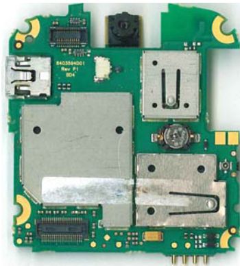
Main PCB (Side B)
