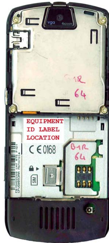
Rear View with Battery Cover Removed Showing ID Label
