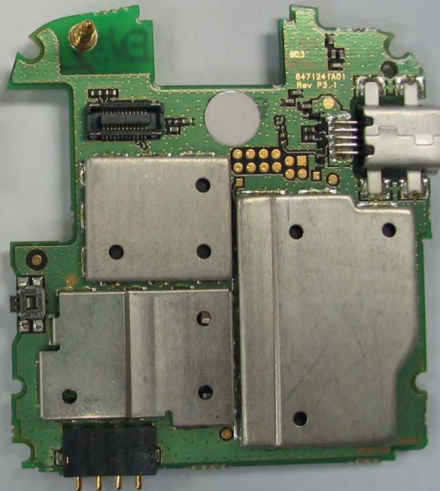
Main PCBA (Rear View)
