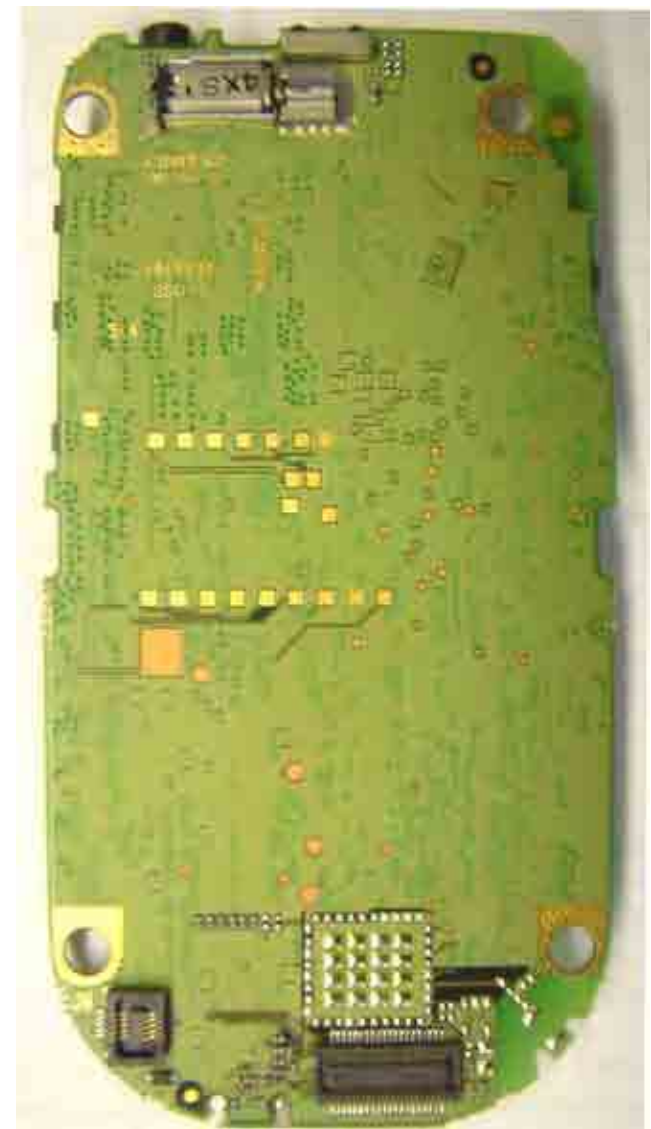
Front View
