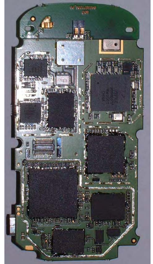
Front View without shields
