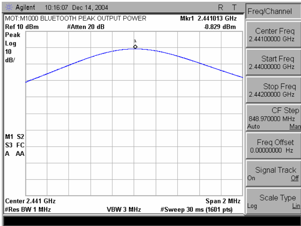
Peak Output Power
